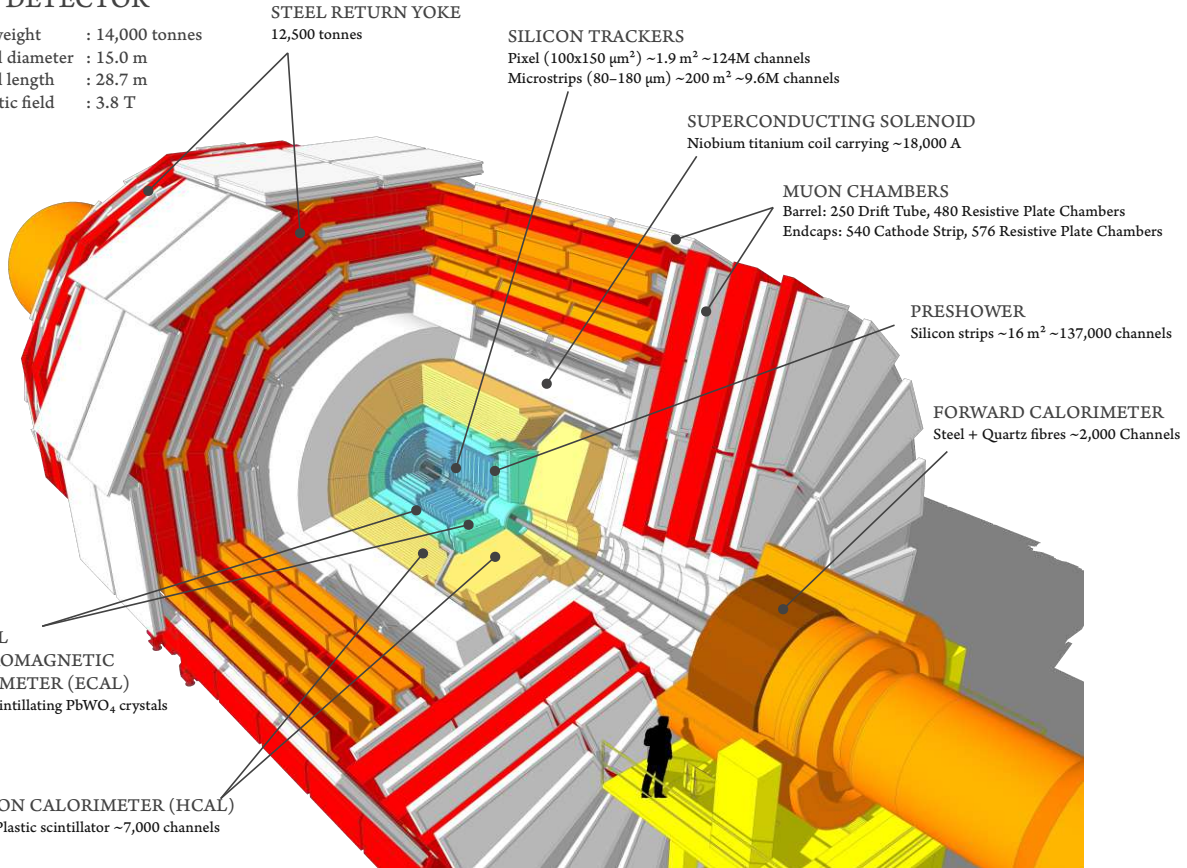
Figure 3.4: A cutaway diagram of the CMS detector along with all the subsystems is shown [38].
