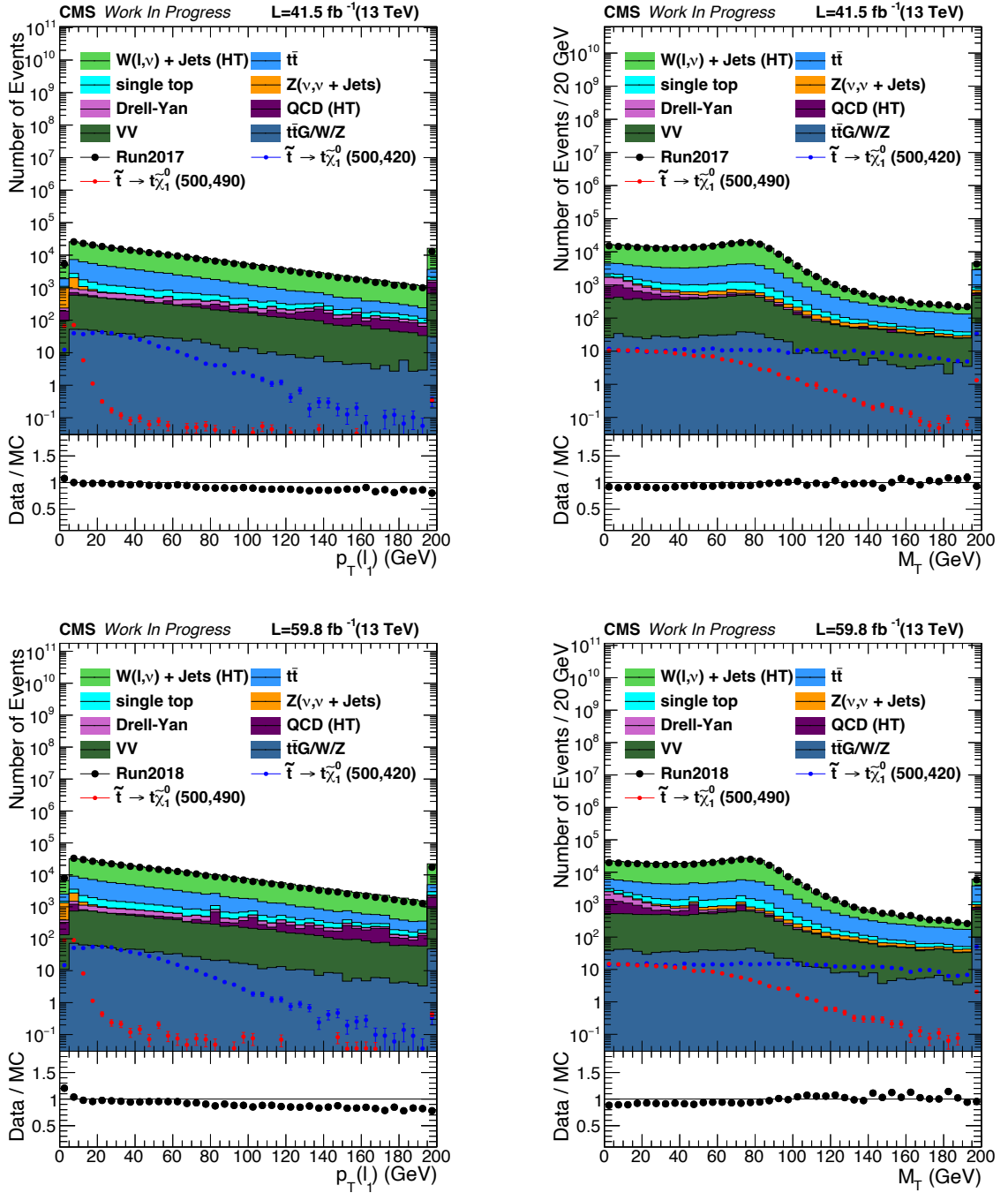
Figure 4.9: Distributions of leading lepton p_T (left) and M_T (right) for events passing the baseline selection criteria as described in Section 4.3.1, shown for 2017 (top) and 2018 (bottom) data-taking periods. These plots validate the modelling of SM background processes and assess data-MC agreement in different periods. Backgrounds are broken down by process, with representative signal benchmarks overlaid for comparison.
