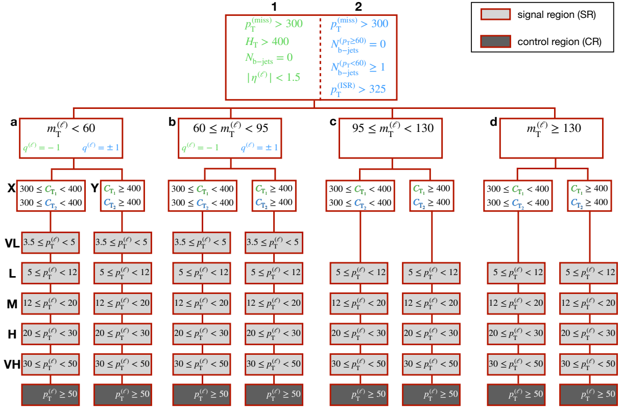
Figure 4.10: The graphic schematic visualizes the splitting of regions into 72 signal regions and 16 control regions, as described in Section 4.4.1 and Section 4.4.2, respectively. Region “1” (green) is predominantly W+Jets, whereas region “2” (blue) has large contributions from W+Jets and t\bar{t} . Each main region is split into four regions, labelled “a” to “d”, depending on M_T selection, and further split into C_{T1} or C_{T2} selections depending on whether it belongs to region “1” or “2”. These are then subdivided into six lepton p_T bins: five low p_T(\ell) bins define the signal regions (“VL”, “L”, “M”, “H”, “VH”) and one high- p_T(\ell) bin used to define control region.
