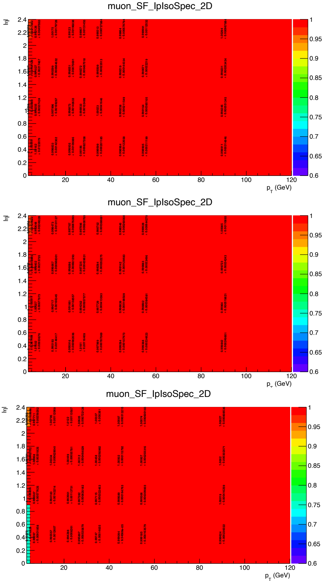
Figure B.2: Muon hybrid isolation and impact parameter scale factors derived privately for the 2016, 2017 and 2018 data-taking periods are shown in the figure.
