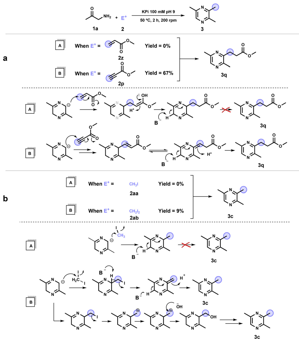
Fig. 4 Tautomerisation experiments. The aromatic character of the final pyrazine product is critical to drive the equilibria towards the products and make the incorporation of the electrophile predominate over the oxidation pathway. Therefore, experiments with methyl acrylate 2z , methyl propioate 2p , iodomethane 2aa and diiodomethane 2ab were carried out to reveal this effect and prove that a tautomerisation step is necessary. This hypothesis is further supported by the deuteration experiments shown in Fig. 3c. The position of the electrophile is represented by the blue circle.
