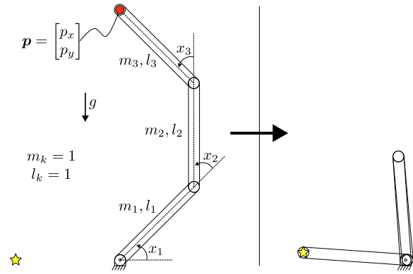
Fig. 2. Left: A three-link planar robot arm system, where the red dot and yellow star represent the initial condition and the desired position, respectively. Right: The result of the optimization problem where the arm folds onto itself to minimize the static torque requirement while satisfying the equality constraint.
