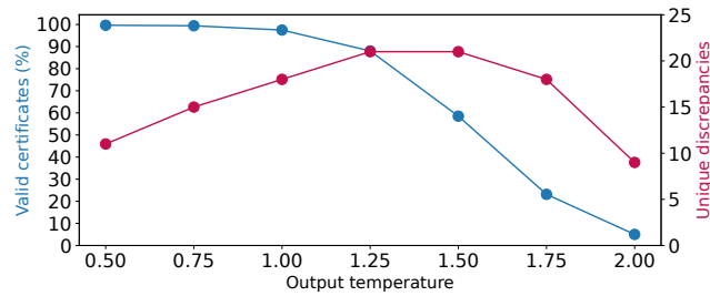
Figure 4: Trade-off between sampling strategy and discrepancies found. Sampling in a conservative way (left) makes more synthetic certificates valid, but they find less discrepancies.
