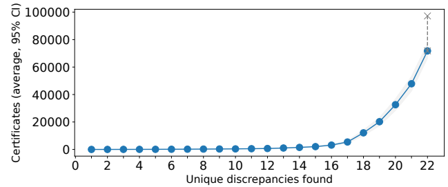
Figure 5: The number of y certificates required to observe x discrepancies with the model IPv4/RNN-Medium. Most unique discrepancies are discovered with just 20,000 synthetic certificates. The gray dashed arrow shows certificates that did not lead to the discovery of new discrepancies.
