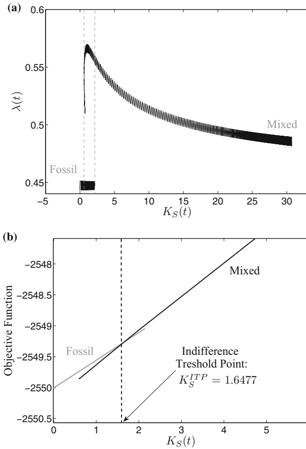
Fig. 4 a Overlap of trajectories leading into the two periodic solutions and b Indifference threshold point: intersection of the objective function values
