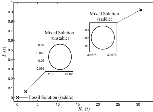
Fig. 2 The three detected periodic solutions in the state-control space
