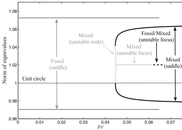
Fig. 10 Norm of eigenvalues of long-run periodic solutions for a fossil energy price p_F \leq 0.07
