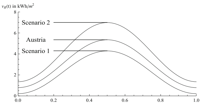
Fig. 12 Deterministic functions for global radiation
