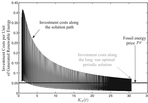
Fig. 6 Investment costs per unit of generated renewable energy along the path leading into the mixed optimal long-run periodic solution
