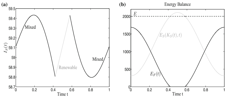
Fig. 9 Mixed-arc solution with two mixed arcs and one renewable arc in between: a Investment I_S(t) and b energy balance
