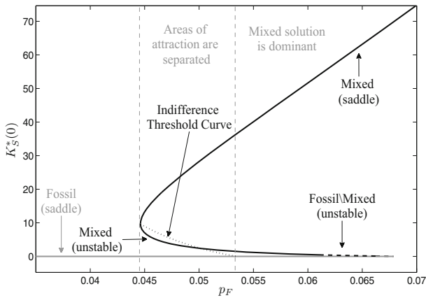
Fig. 7 Bifurcation diagram with respect to a fossil energy price p_F \leq 0.07
