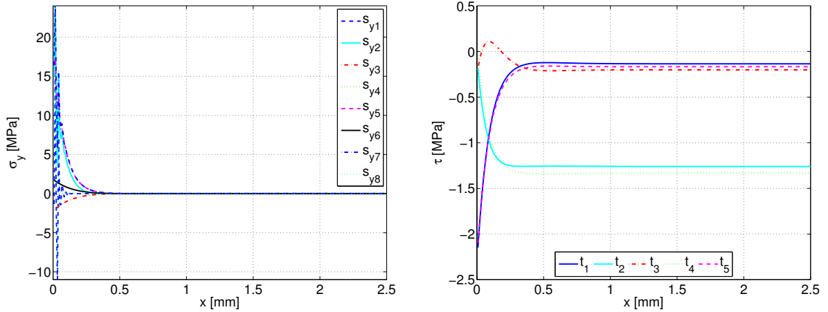
Figure 6. Transverse compressive stress \hat{\sigma}_y (left) and shear stress \hat{\tau} (right) as functions of x for a three-layer homogeneous cantilever, clamped at x = 0 , loaded at x = 2.5 by a quadratic shear distribution, and modeled with 64 elements.
