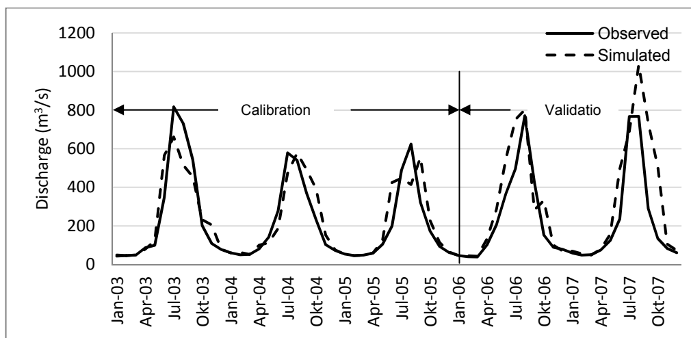
Figure A-4 Observed and simulated discharge at station No. 684 in the Koshi basin (Source: Author)
