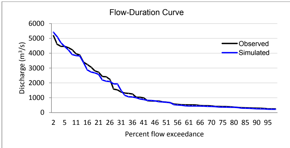
Figure 22: FDC of the observed and simulated flow at station No. 280 in the Karnali basin (Source: Author)
