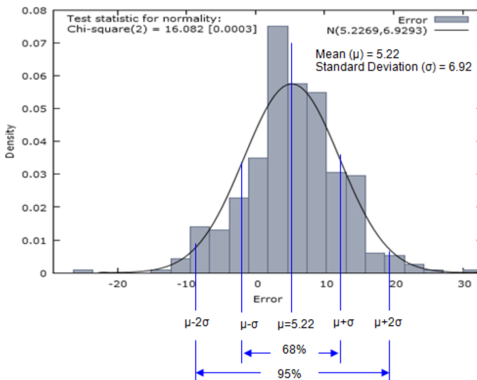
Figure 23: Error histogram with normality test and confidence interval for the flow exceedance \geq 30\% (Source: Author)
