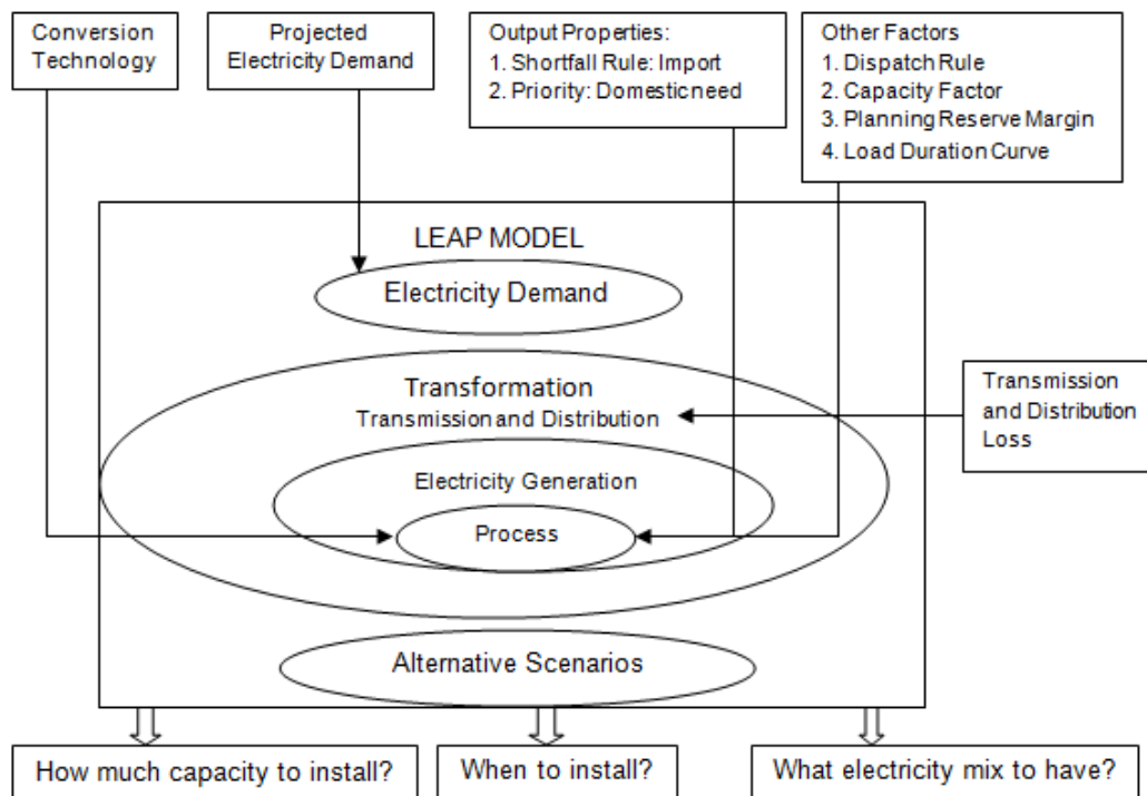
Figure 9: LEAP model for power generation and expansion planning (Source: Author)
