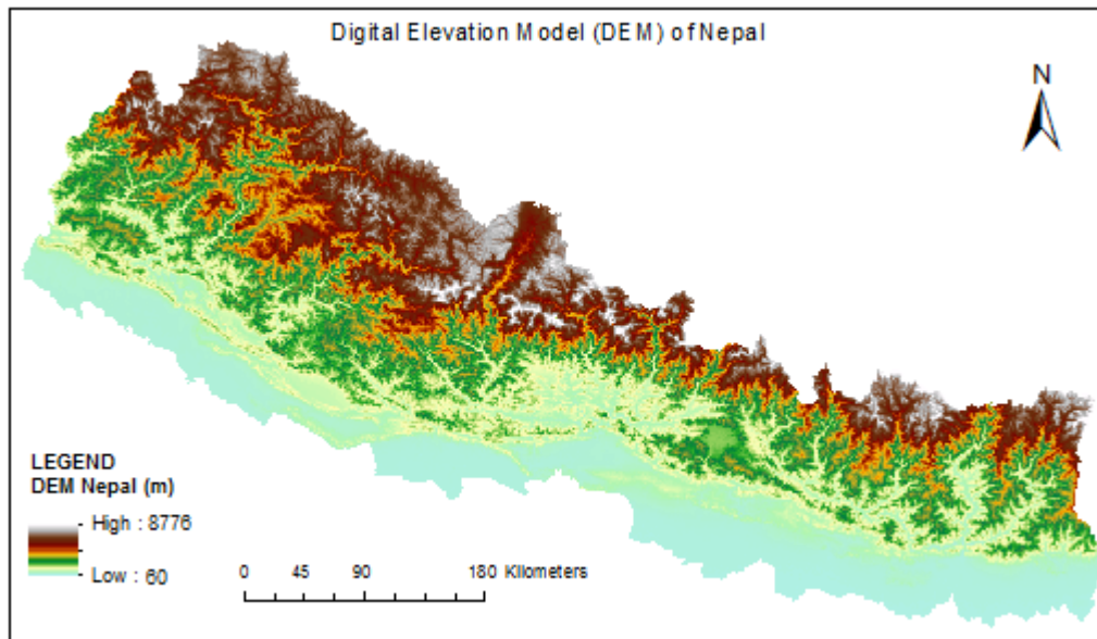
Figure 11: Projected Digital Elevation Model of Nepal (Source: Author)
