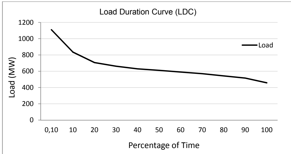
Figure 41: Load duration curve for the year 2012 (Source: NEA)
