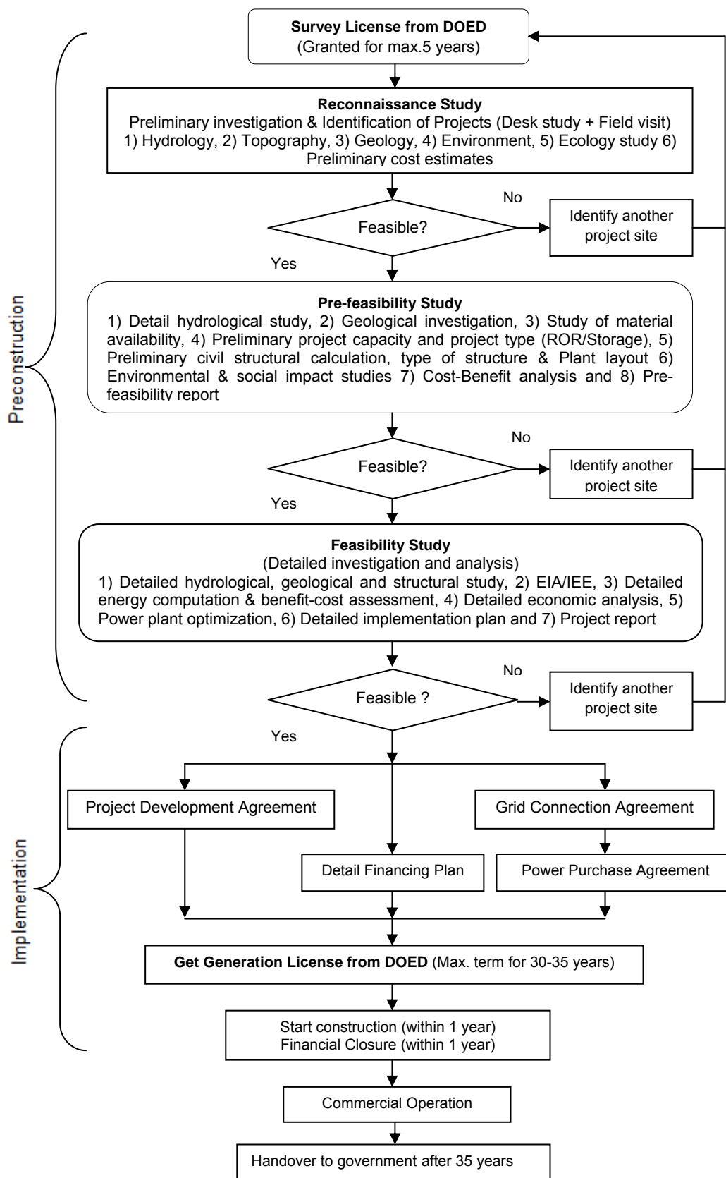
Figure 25: Flowchart for hydropower project development process in Nepal [149, 150]
