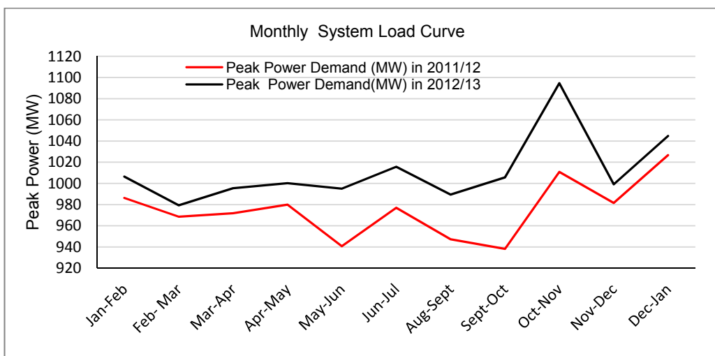
Figure 31: Monthly peak power demand curve (Source: NEA)
