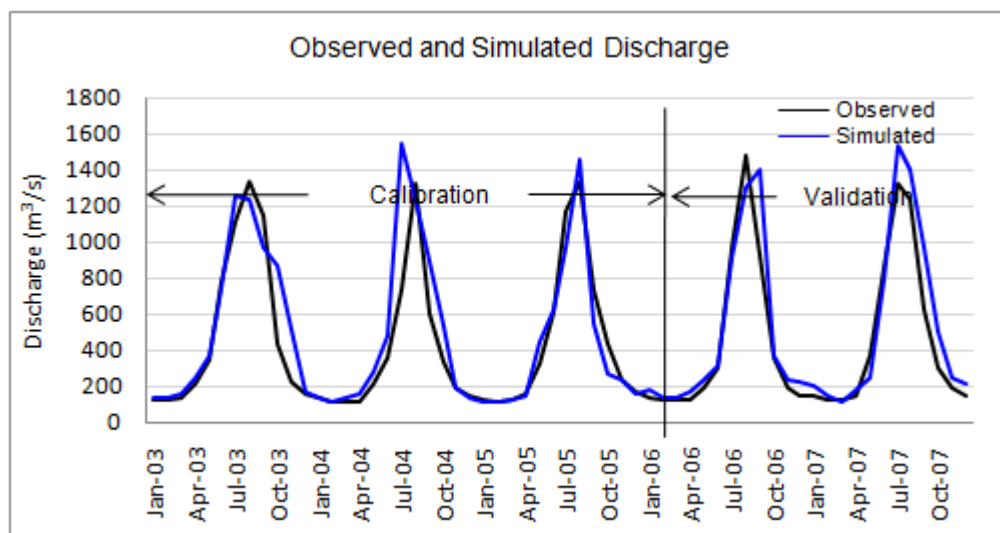
Figure 19: Observed and simulated discharge at station No. 240 in the Karnali basin (Source: Author)
