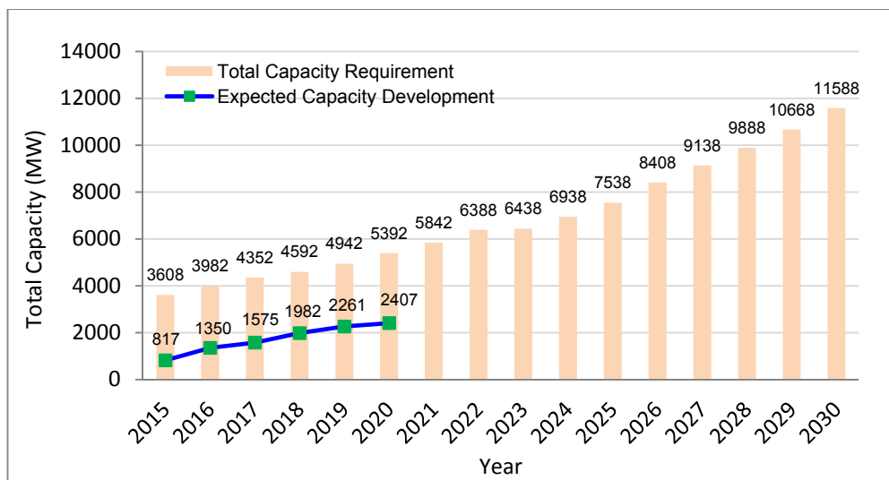
Figure 46: PS capacity requirement for medium growth electricity demand (Source: Author)
