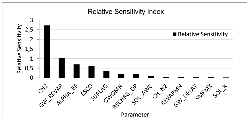
Figure 14: Sensitive parameters and their relative sensitivities in the Karnali basin outlet (Source: Author)
