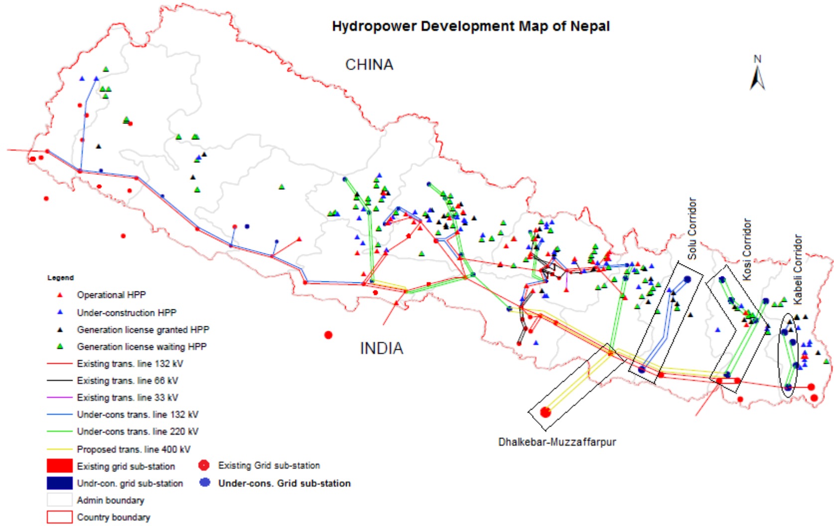
Figure 34: Hydropower development map of Nepal Diagram extended from Annual Review, NEA, 2014
