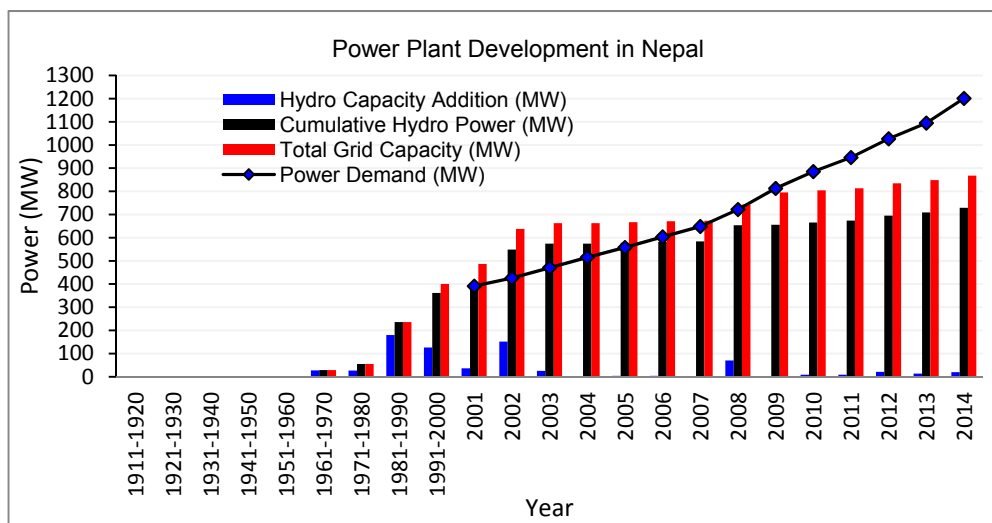
Figure 33: Power Plant Development in Nepal [73, 161, 162]
