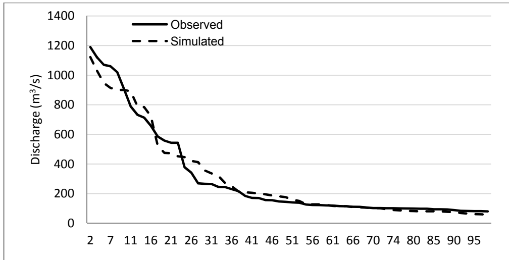
Figure A-16: FDC for observed and simulated flow at station No. 269.5 in the Karnali basin (Source: Author)
