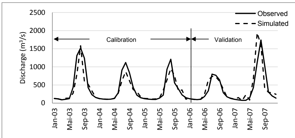
Figure A-6: Observed and simulated discharge at station No.420 in the Narayani basin (Source: Author)
