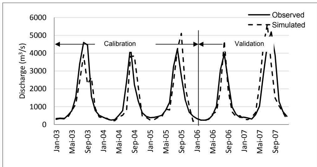
Figure A-9: Observed and simulated discharge at station No.280 in the Karnali basin (Source: Author)
