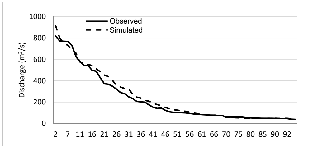
Figure A-11: FDC for observed and simulated flow at station No. 684 in the Kosi basin (Source: Author)
