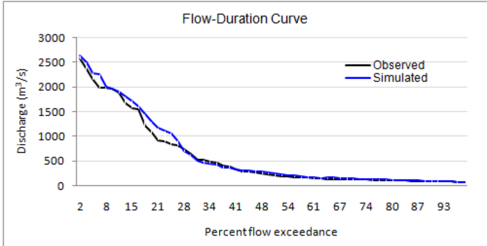
Figure 20: FDC of the observed and simulated flow at station No. 652 in the Koshi basin (Source: Author)
