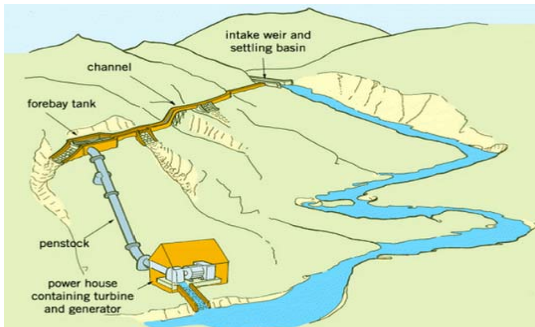
Figure 26: Typical ROR plant with open channel [157]
