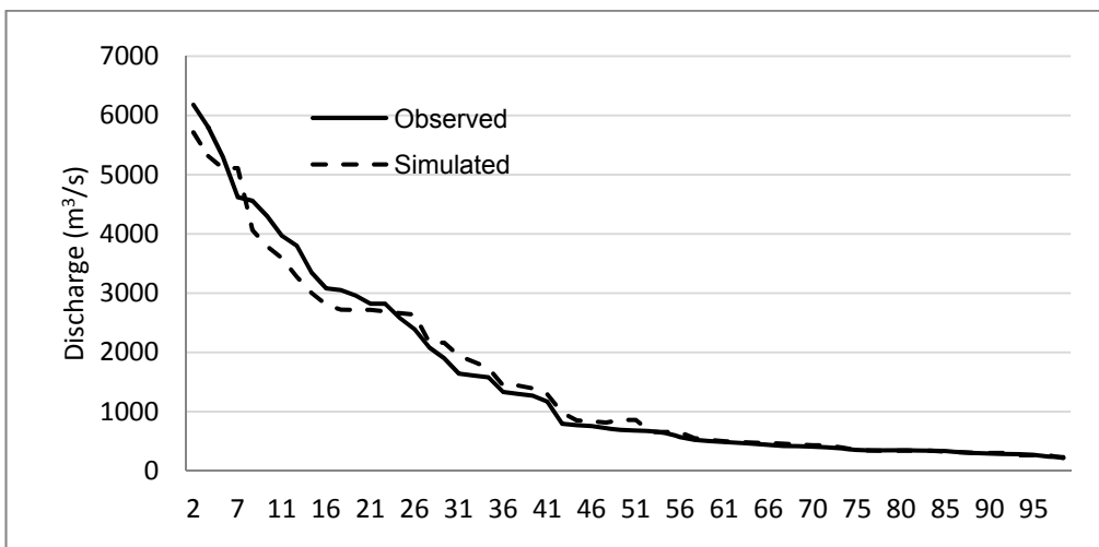
Figure A-12: FDC for observed and simulated flow at station No. 695 in the Koshi basin (Source: Author)
