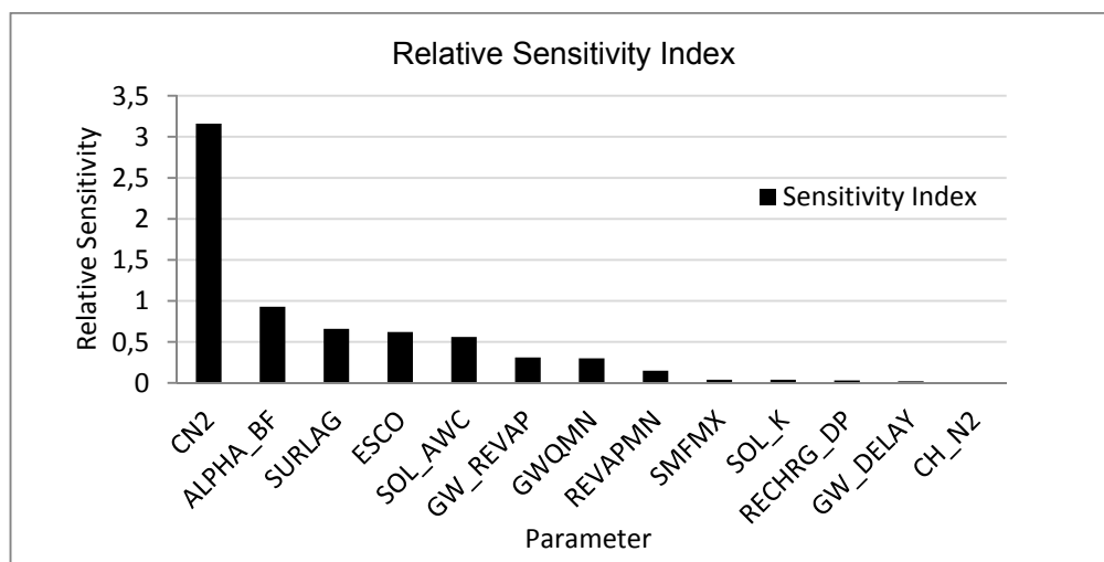
Figure 15: Sensitive parameters and their relative sensitivities in the Narayani basin outlet (Source: Author)
