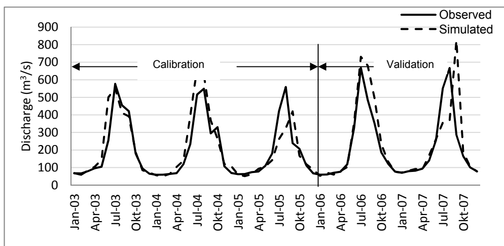
Figure A-3: Observed and simulated discharge at station No. 600.1 in the Koshi basin (Source: Author)
