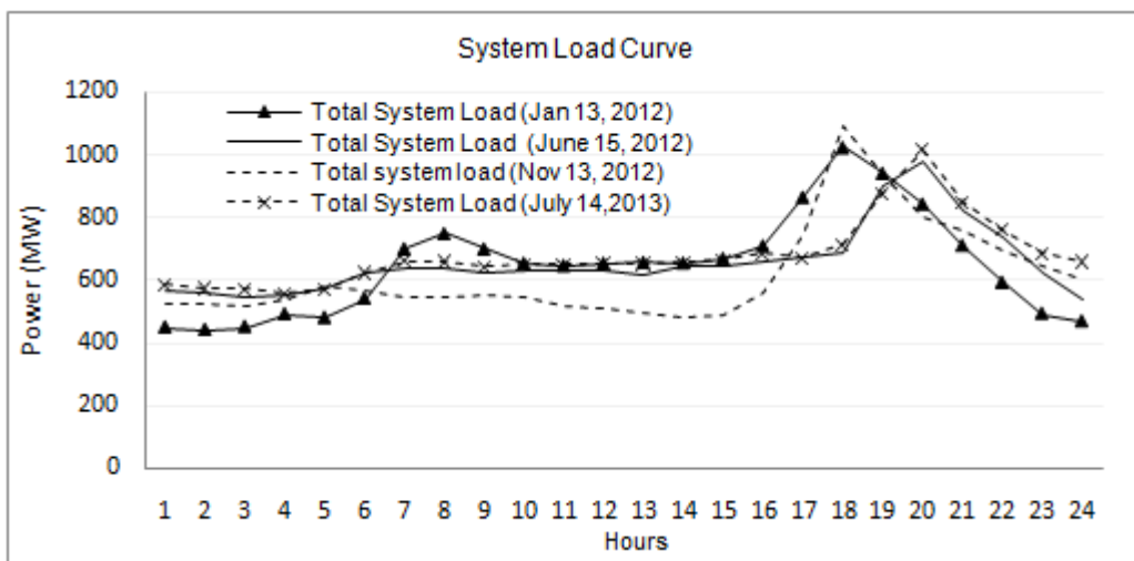
Figure 30: Hourly system load curve of peak load day in Nepal (Source: NEA)
