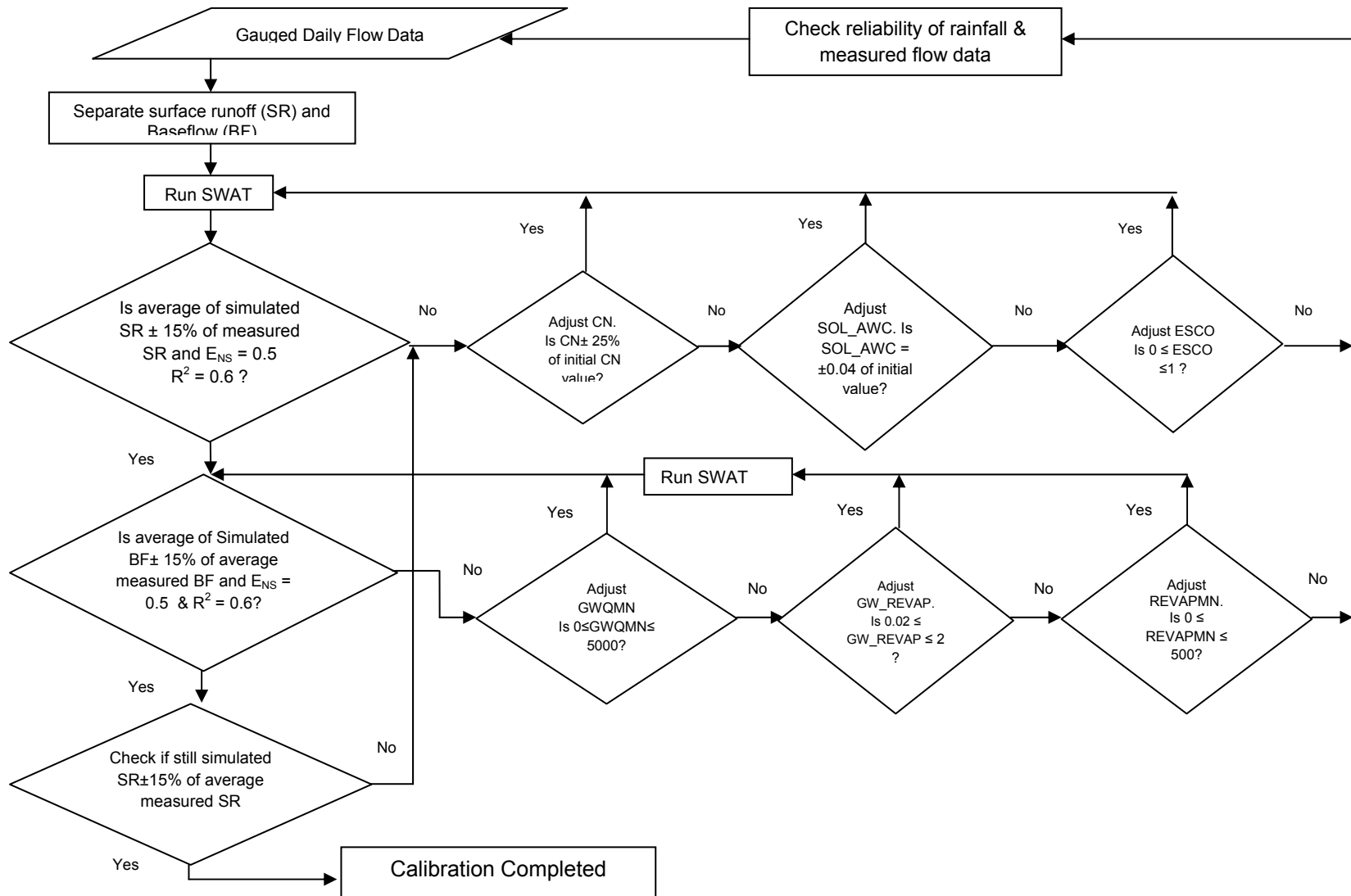
Figure 16: Manual calibration process flowchart used in this study. Diagram extended from [65, 134, 138]
