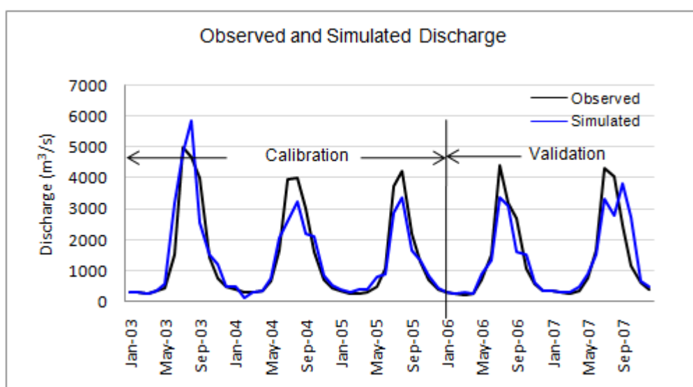
Figure 18: Observed and simulated discharge at station No. 450 in the Narayani basin (Source: Author)
