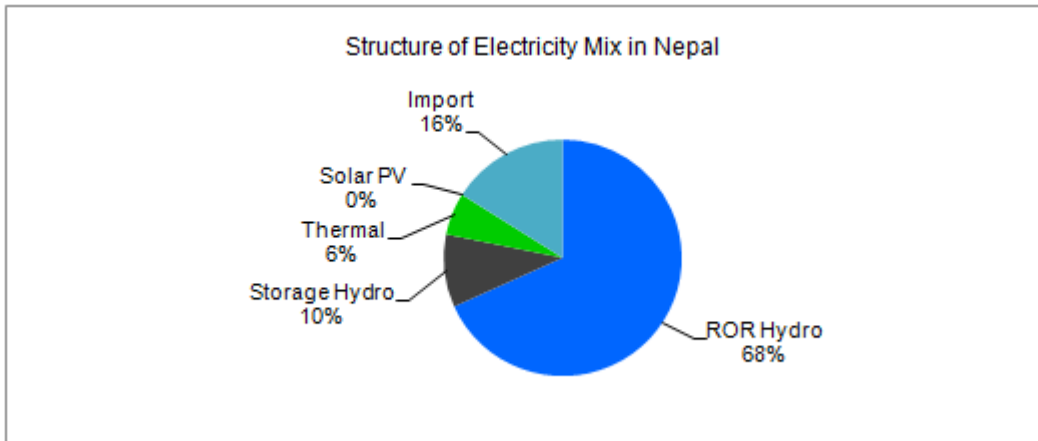
Figure 32: Structure of Electricity Mix in Power System of Nepal (Source: NEA)
