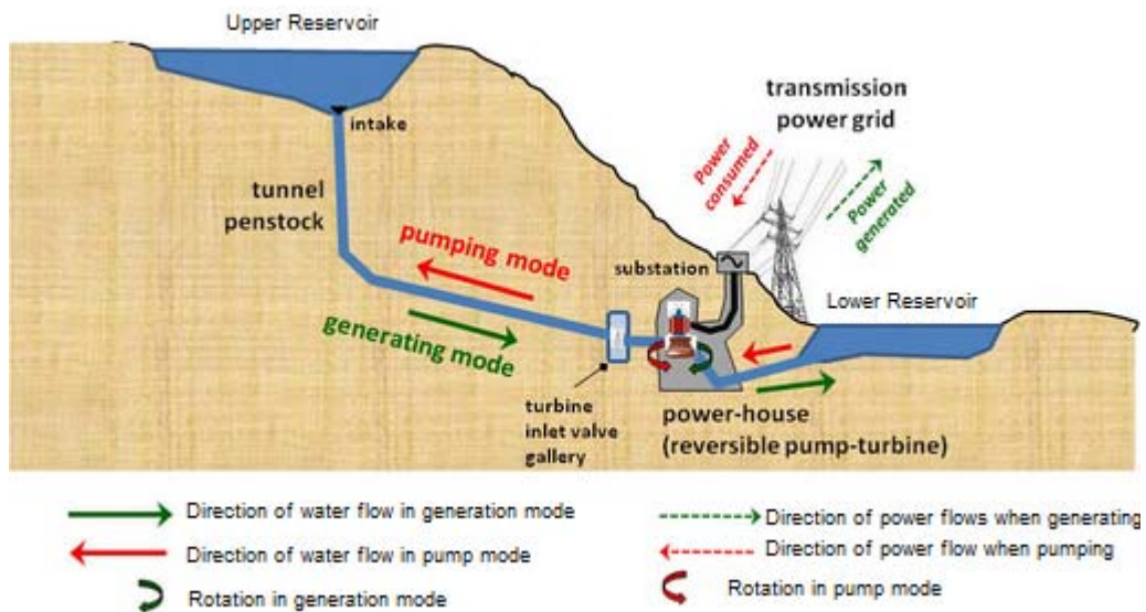
Figure 28: Typical pump storage hydropower plant [159]
