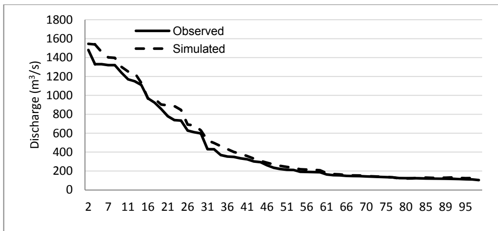
Figure A-15: Flow duration curve for observed and simulated flow at station No. 240 in the Karnali basin (Source: Author)
