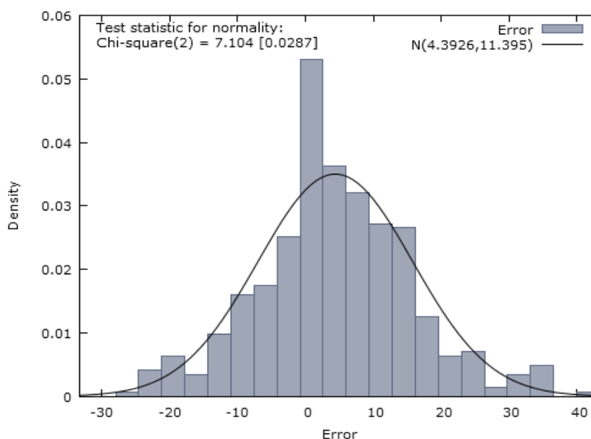
Figure A-18: Error histogram of the flow variation between observed and simulated flow for the entire FDC (Source: Author)
