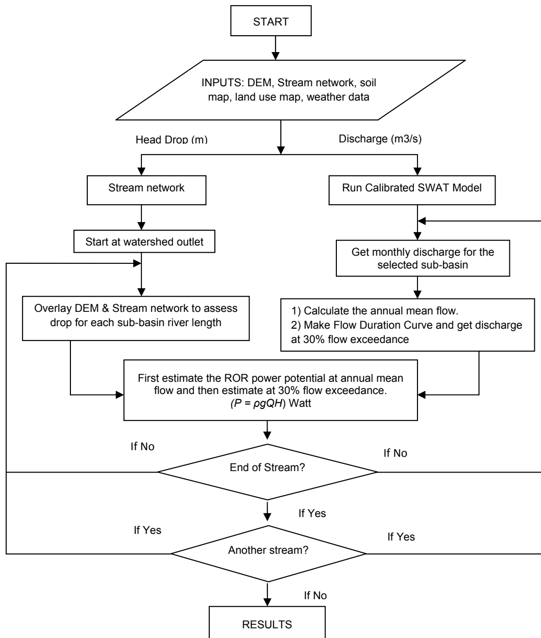
Figure 5: Flow chart for estimation of theoretical ROR hydropower potential Diagram extended from Kurse, 2010.
