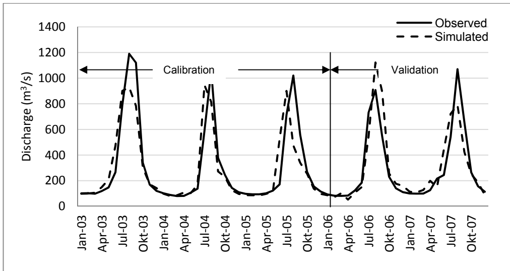
Figure A-8: Observed and simulated discharge at station No.269.5 in the Karnali basin (Source: Author)
