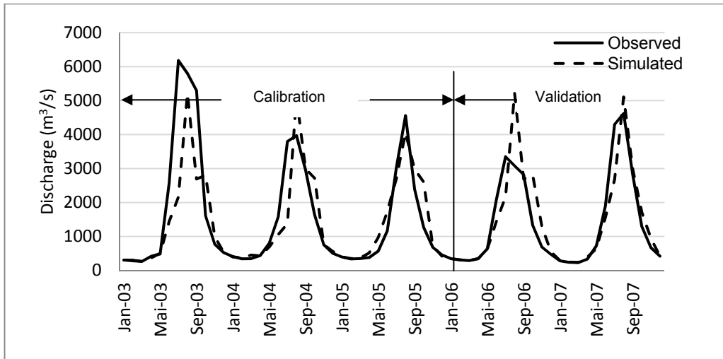
Figure A-5: Observed and simulated discharge at station No.695 in the Koshi basin (Source: Author)
