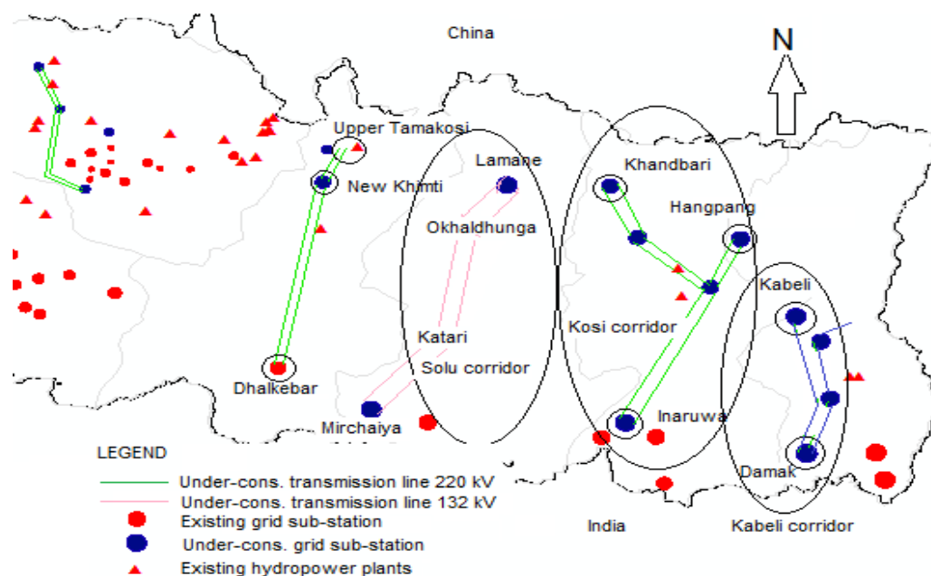
Figure 35: Location of different under-construction transmission line (Source:NEA)
