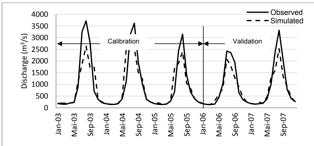
Figure A-7: Observed and simulated discharge at station No.449.91 in the Narayani basin (Source: Author)
