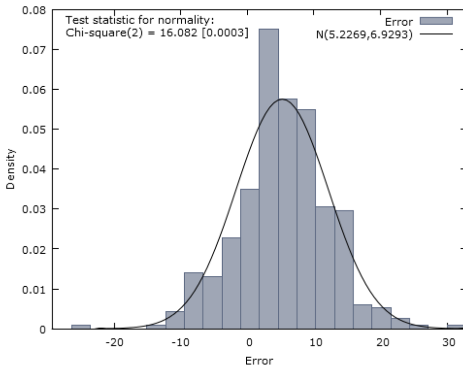
Figure A-17: Error histogram of the flow variation between observed and simulated flow for the flow exceedance \geq 30\% in FDC (Source: Author)
