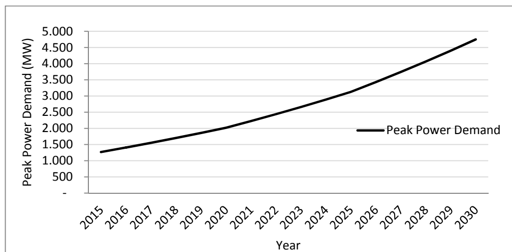
Figure 49: Peak power demand for high growth electricity demand (Source: Author)
