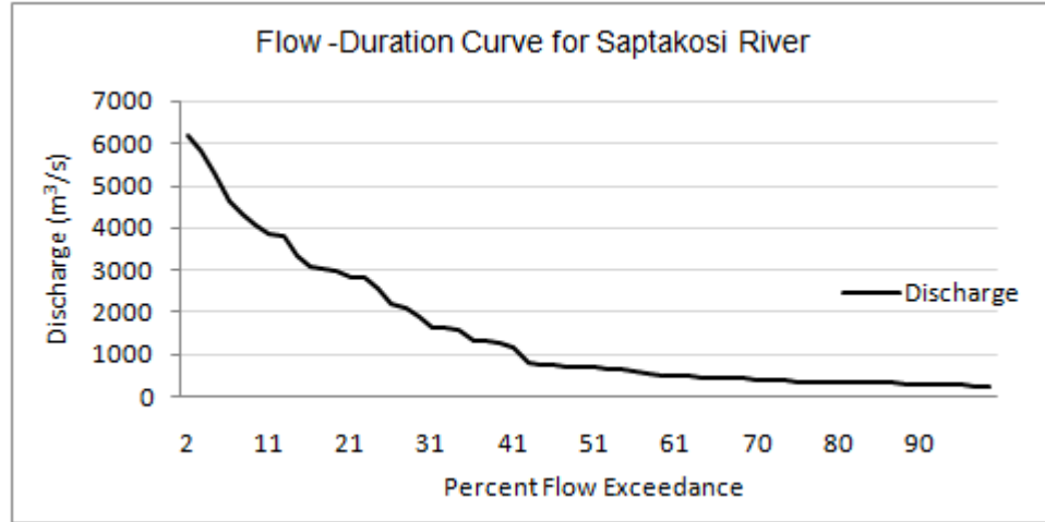
Figure 6: A typical flow duration curve of the Saptakoshi River in Nepal (Source: Author)
