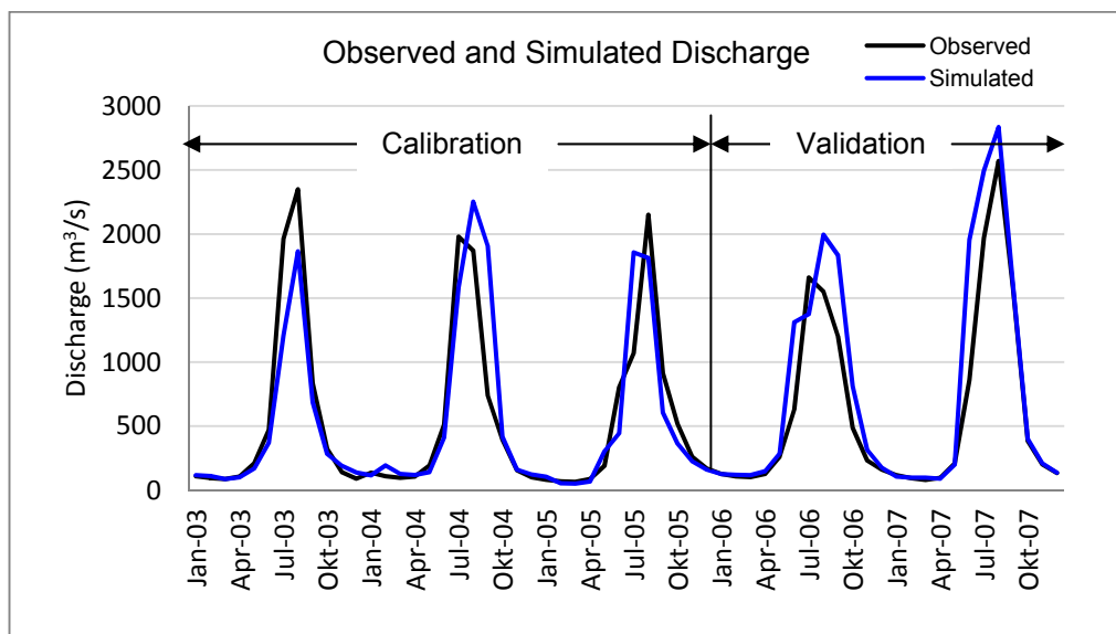
Figure 17: Observed and simulated discharge at station No. 652 in the Koshi basin (Source: Author)
