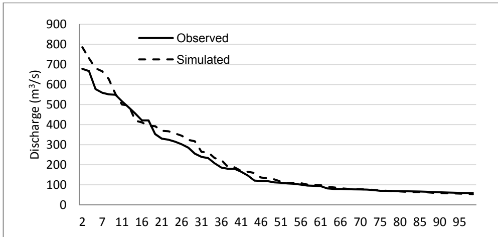
Figure A-10: FDC for observed and simulated flow at station No. 600.1 in the Kosi basin (Source: Author)
