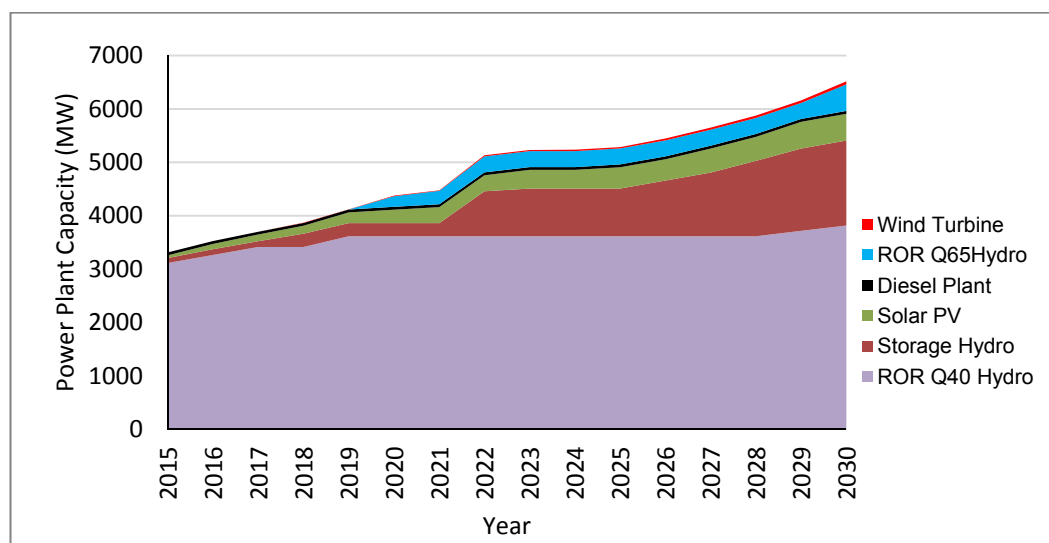
Figure 45: Structure of Electricity Mix Scenario (Source: Author)
