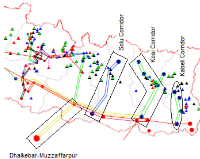
Figure 38: Location of Dhalkebar-Muzaffarpur and Solu corridor transmission lines (Source: NEA)
