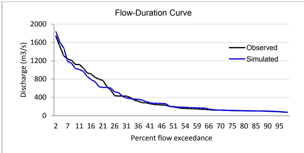
Figure 21: FDC of the observed and simulated flow at station No. 420 in the Narayani basin (Source: Author)
