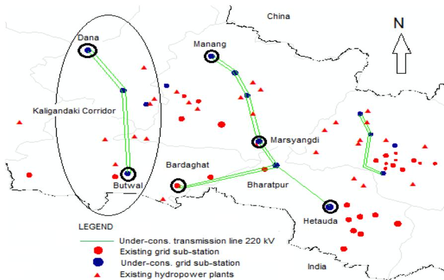
Figure 37: Location of 220 kV under-construction transmission line (Source: NEA)
