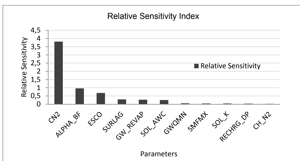
Figure 13: Sensitive parameters and their relative sensitivities in the Koshi basin outlet (Source: Author)
