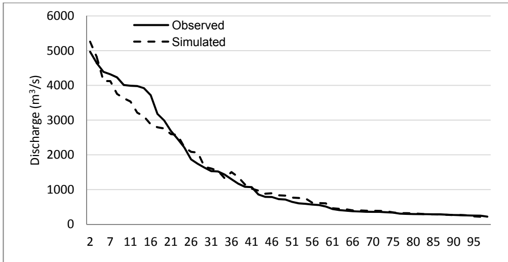
Figure A-13: FDC for observed and simulated flow at station No. 450 in the Narayani basin (Source: Author)
