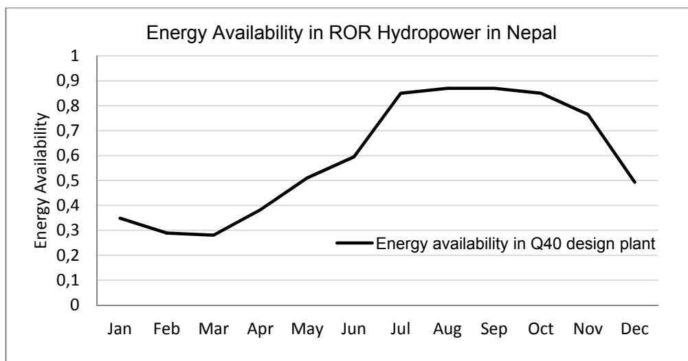
Figure 42: Average energy availability from ROR hydropower plant in Nepal (Source: NEA)
