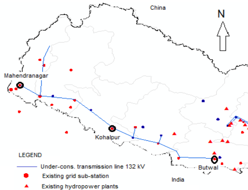
Figure 36: Location of Butwal-Kohalpur-Mahendranagar transmission line (Source:NEA)
