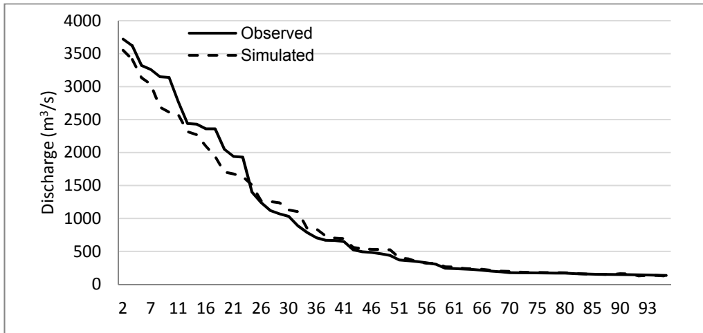
Figure A-14: FDC for observed and simulated flow at station No. 449.1 in the Narayani basin (Source: Author)
