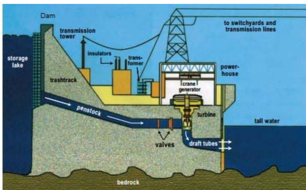
Figure 27: Typical storage hydropower plant with powerhouse at dam toe [158]
