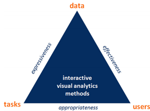
Figure 1.7: Design triangle [274]
