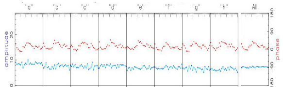
Figure 7: Correlation amplitude and phase vs. time for first 8 channels of observation in Figure 6.
