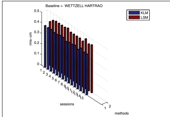
Figure 1. Formal errors for estimated baseline lengths for simulated CONT05 sessions
