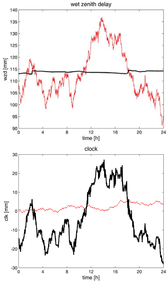
Fig. 3a Impact of the a priori process noise variance of wet zenith delay on the estimation: The upper figure shows the wet zenith delay, the lower figure shows the station clock. The a priori process noise variance of wet zenith delay was chosen as 0.0001 \text{ mm}^2 which is too low. Red (thin) lines: simulated data, black (bold) lines: estimation.
