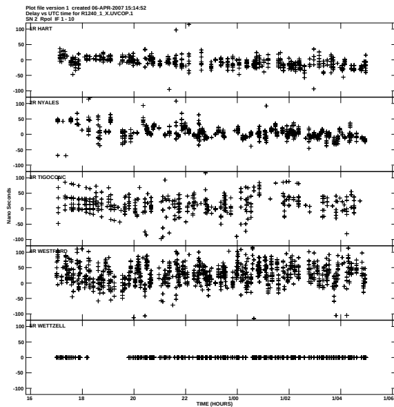
Figure 3. Delay residual in X-band of a single-channel antenna-based fringe fit. The reference station Wettzell has fixed zero delay. Due to the low SNR the scatter in the delay solutions is fairly high.
