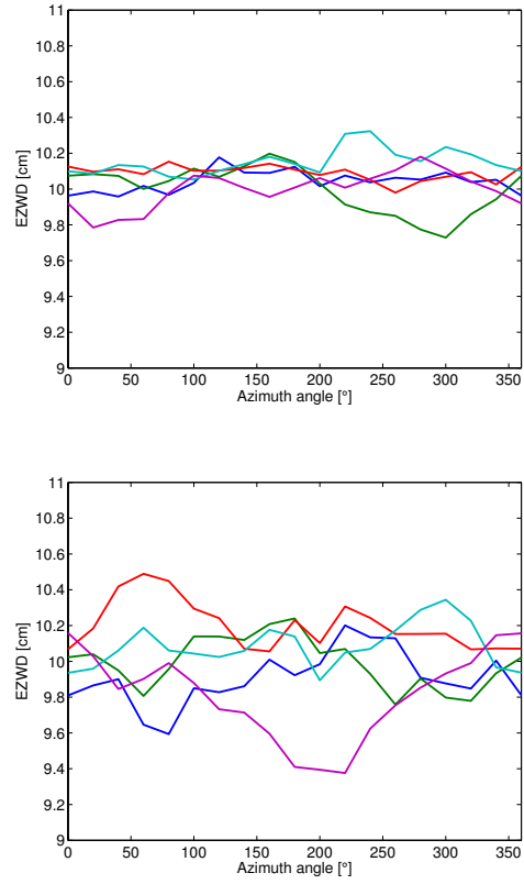
Figure 2. Simulated EZWDs for elevation angle 45^\circ (top) and 10^\circ (bottom) as function of azimuth angle. The results of five different simulations are shown for each elevation angle, represented by the different lines. Note that the variations seen along the simulated azimuth scan in the actual direction of observation is approximately 1.4 and 6 times larger at the 45^\circ and the 10^\circ elevation angle, respectively.
