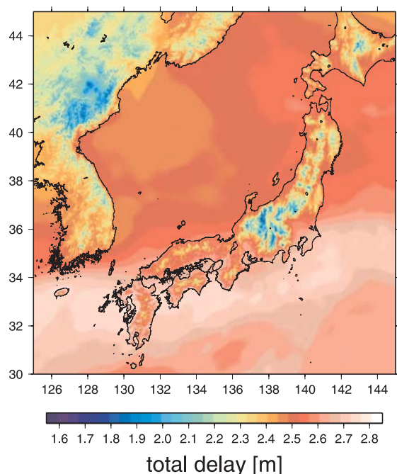
Figure 1. Total zenith delay on July 23, 2006 00UT obtained from ray-tracing through the 10km mesoscale model.
