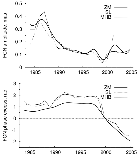
Figure 1. Variation of the FCN amplitude and phase in accordance with three FCN models.
