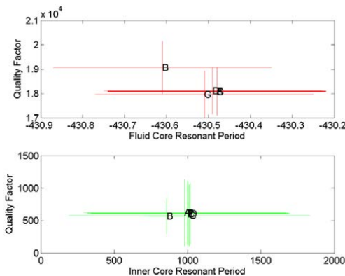
Fig. 3. RFCN and FICN frequencies and quality factors obtained through solutions A to G.
