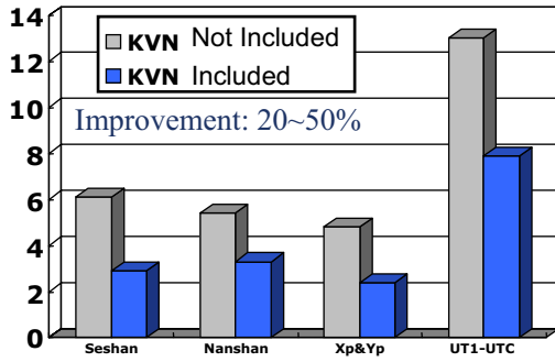
Fig. 2 The formal errors of station coordinates and EOP analysis for KVN-Asia (Unit : 3-D coordinates(mm), Xp&Yp( \mu\text{as} \times 100 ), UT1-UTC( \mu\text{s} )).
