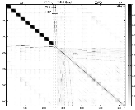
Figure 2. Correlation matrix of session 05SEP19XA with NNR/NTT conditions.
