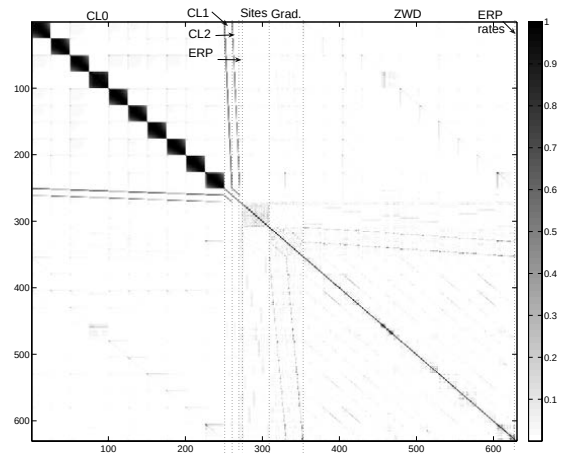
Figure 4. Correlation matrix of session 05SEP19XA of the complete solution with NNR/NTT conditions. Only an extract of parameters valid for this session is displayed.
