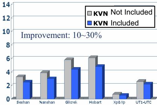
Fig. 3 The formal errors of station coordinates and EOP analysis in KVN-Pacific (Unit : 3-D coordinates(mm), Xp&Yp( \mu\text{as} \times 100 ), UT1-UTC( \mu\text{s} )).
