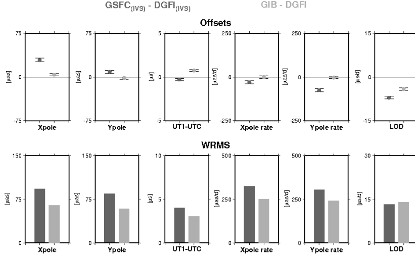
Figure 5. Results of EOP comparisons of the different VLBI solutions, offsets and WRMS for \text{GSFC}_{\text{IVS}} - \text{DGFI}_{\text{IVS}} differences (left column) and \text{GIB} - \text{DGFI} differences (right column)
