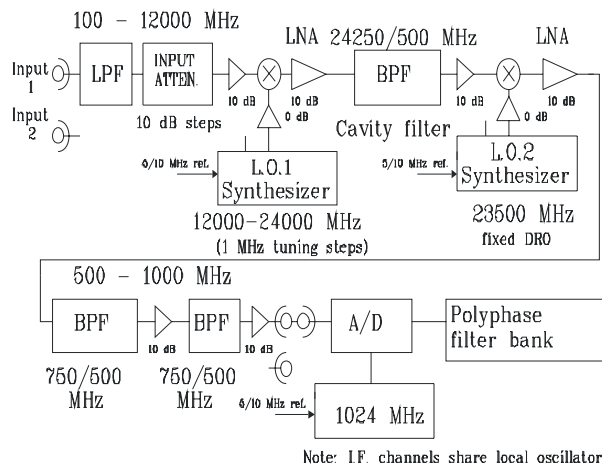
Figure 8: Block diagram of IF-to-baseband converter module (also shows attached A/D converter and PFB)
