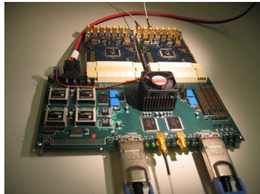
Figure 4: iBOB board with two attached sampler-module boards
