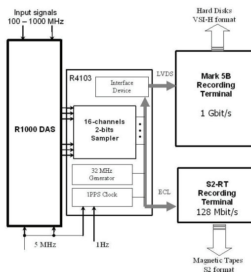
Fig. 1. Block diagram of the VLBI Terminal in Badary Observatory.
