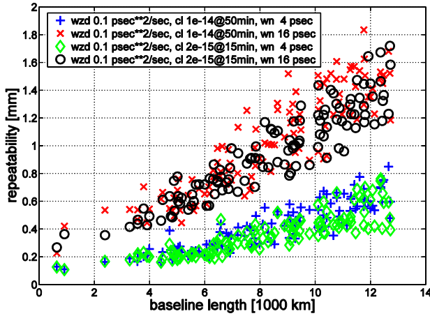
Fig. 5. Baseline length repeatabilities with wet zenith delays that correspond to a PSD of 0.1 \text{ psec}^2/\text{sec} : 4 psec white noise and an ASD of 1 \cdot 10^{-14} @ 50\text{min} for clocks (+); 4 psec white noise and an ASD of 2 \cdot 10^{-15} @ 15\text{min} for clocks ( \diamond ); 16 psec white noise and an ASD of 1 \cdot 10^{-14} @ 50\text{min} for clocks (x); 16 psec white noise and an ASD of 2 \cdot 10^{-15} @ 15\text{min} for clocks ( \circ ).
