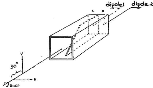
Figure 3. Polarizer operation.
