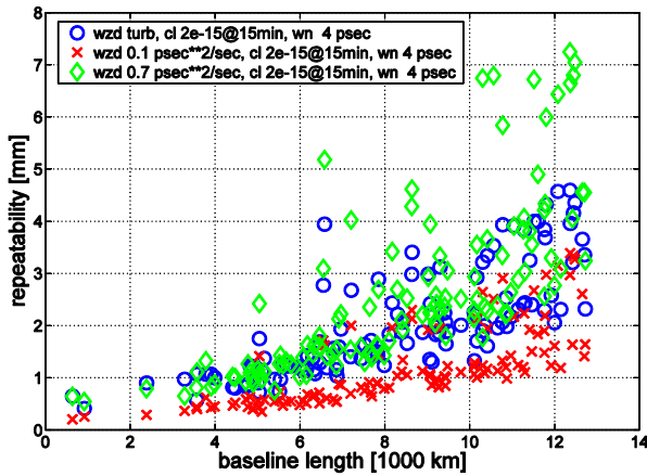
Fig. 6. Baseline length repeatabilities with 4 psec white noise and an ASD of 2 \cdot 10^{-15} @ 15\text{min} for clocks with WZD from the turbulence model ( \circ ), with WZD from the random walk model that correspond to a PSD of 0.1 \text{ psec}^2/\text{sec} (x) and a PSD of 0.7 \text{ psec}^2/\text{sec} ( \diamond ).
