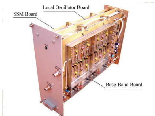
Fig.4. R1200 Base Band Converter.
