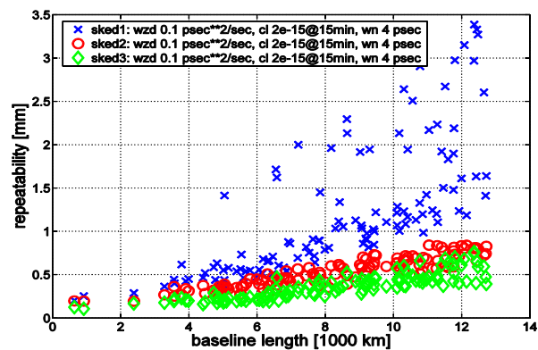
Fig. 2. Baseline length repeatabilities comparing three different schedules (sked1: 57595 observations (x), sked2: 116308 observations (o), and sked3: 226639 observations (o)).
