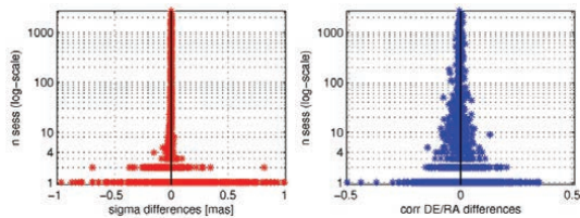
Fig. 3.7 Left: Differences between the lengths of the vectors for the formal errors of two CRF solutions; Right: Differences between the absolute values of the DE/RA correlation coefficients of two CRF solutions. Both display “using elevation dependent weighting – without using elevation dependent weighting” solution differences.
