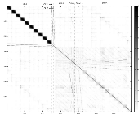
Figure 6. Correlation matrix of a solution with hourly ERP of a independent NNR/NTT solution. The changes to the correlation matrix of a solution with fixed sites or the complete approach are similar to the daily case (Fig. 3 and 4).
