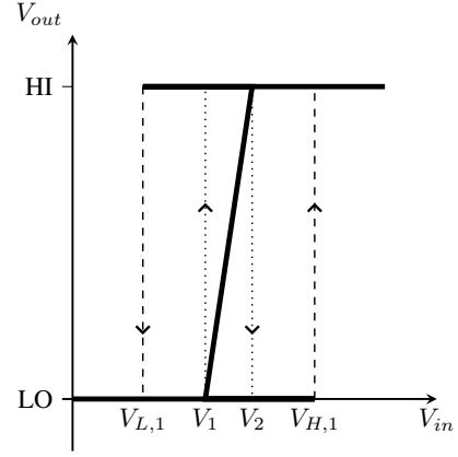
Fig. 7. Theoretical hysteresis ( V_{in} - V_{out} ) of S/T cascade
