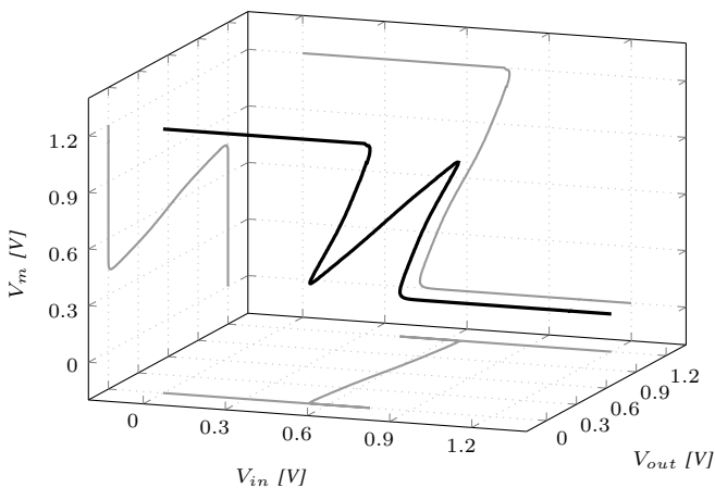
Fig. 14. Characteristic of the cascade
