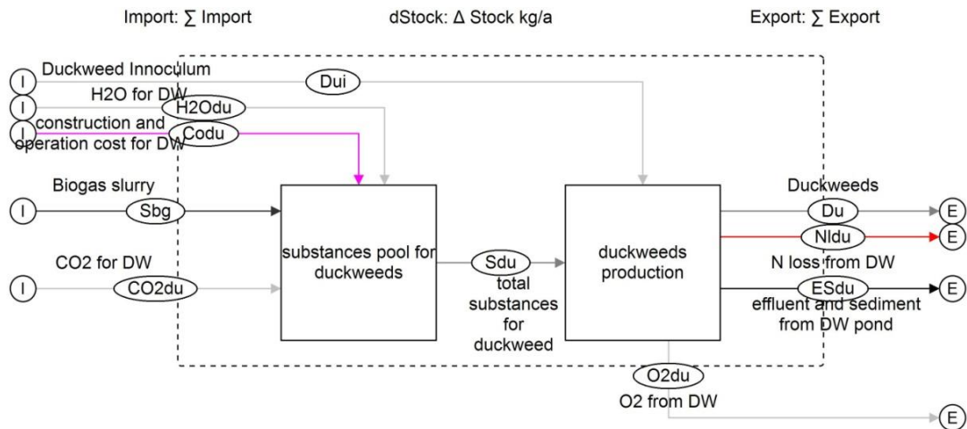
Fig. 3.18. Subsystem of Process "Duckweeds"
