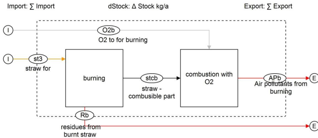
Fig. 3.3. Subsystem in process "RSOB"
