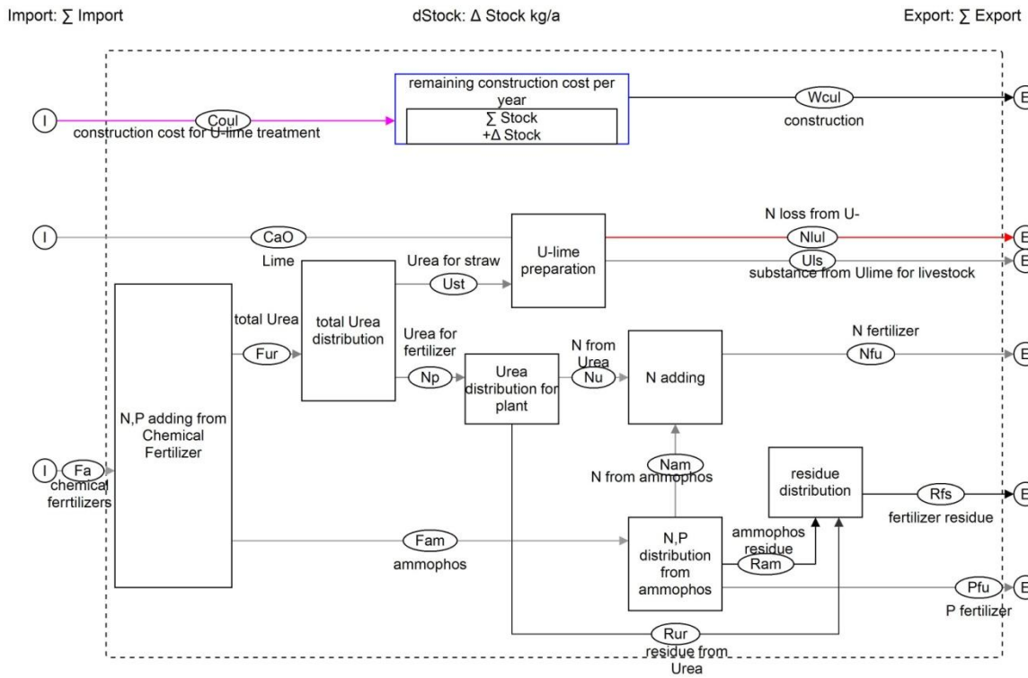
Fig. 3.10. Subsystem of process "Chemical Distribution"
