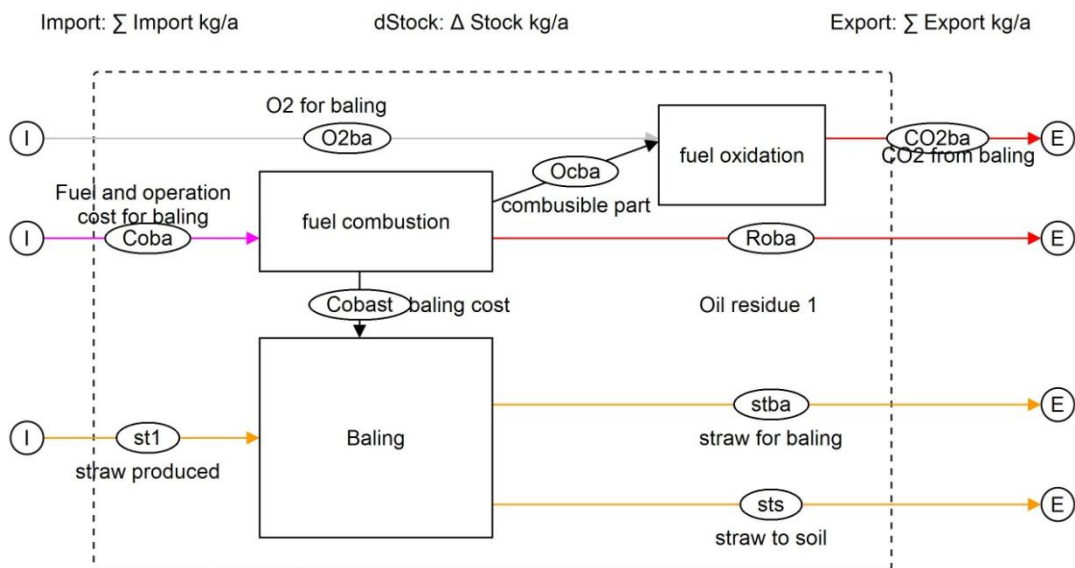
Fig. 3.8. Subsystem Process "Baling"
