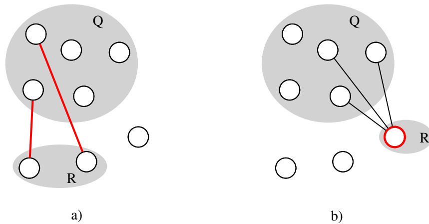
Figure 5.2: Circles denote clusters and a connection between them denote a conflict. ILLP1 would choose a solution with 2 conflicts (a) over a solution with 3 conflicts, which produces fewer conflicting clusters (b).
