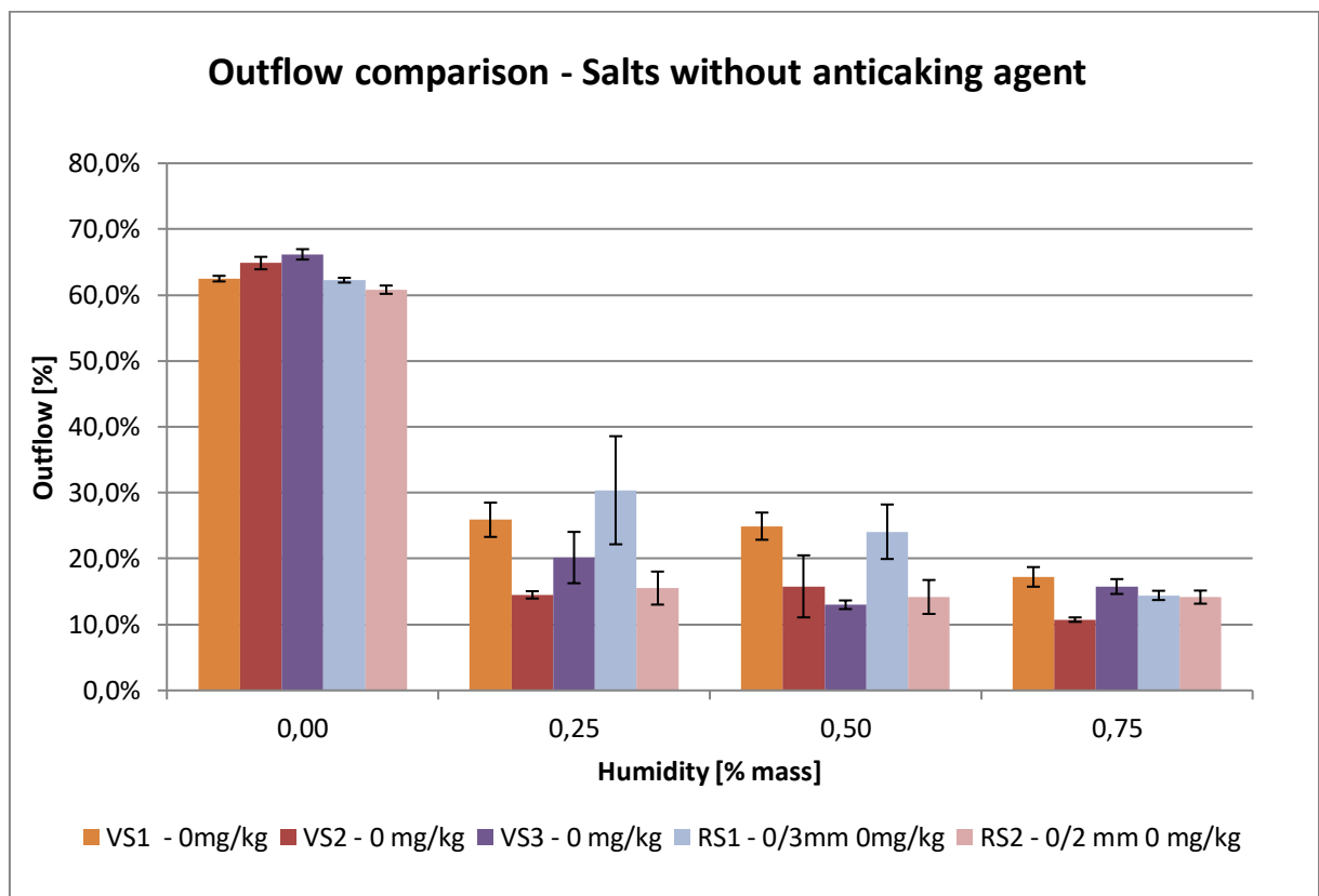
Figure 53: Outflow ratio comparison for salts without anticaking agent
