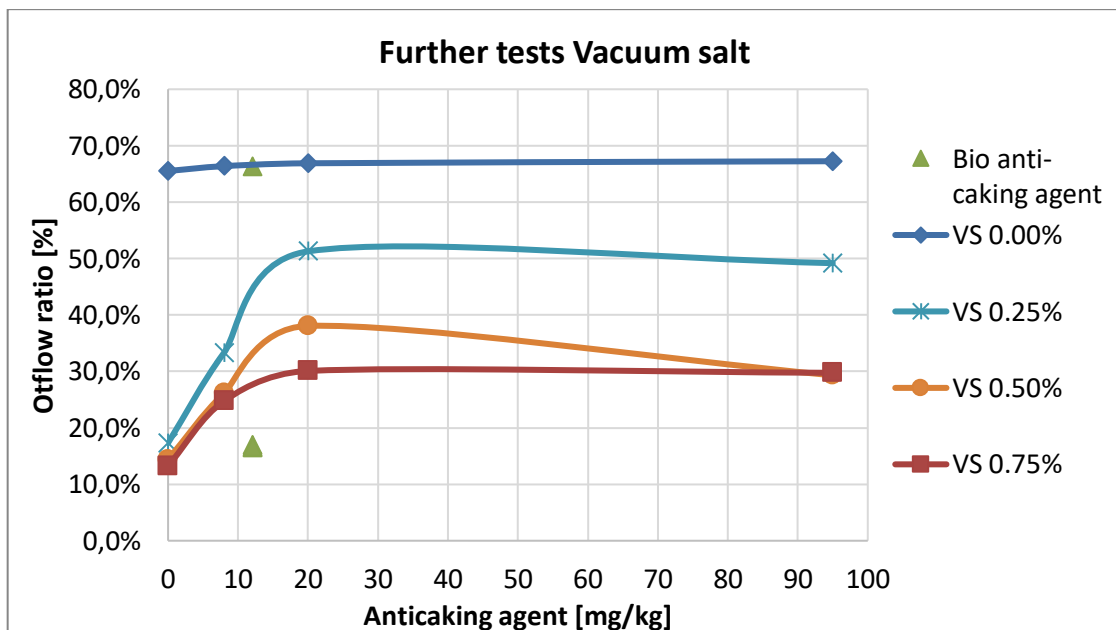
Figure 61: Offflow ratio for VS depending on the amount of anti-caking agent for humidities 0,00 %; 0,25 %; 0,50% and 0,75%
