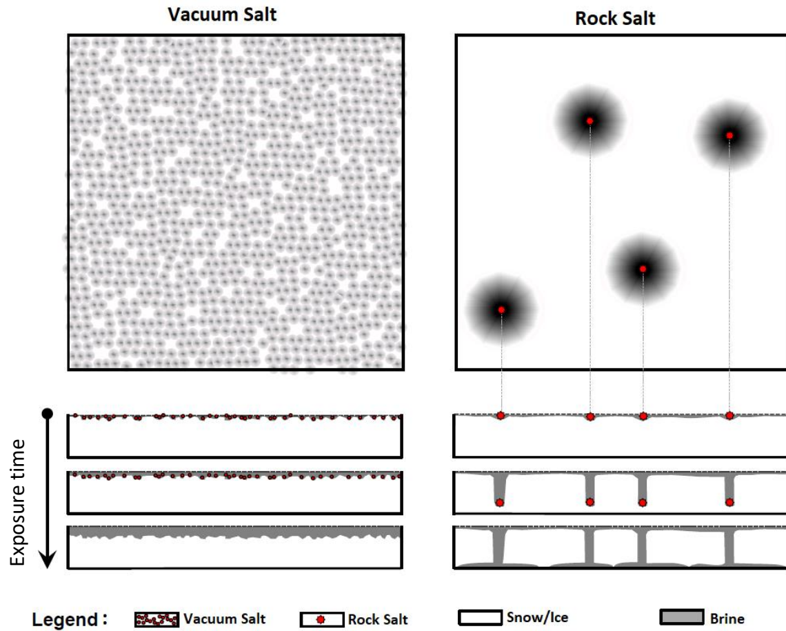
Figure 2. Influence of the grain size in thawing [4]
