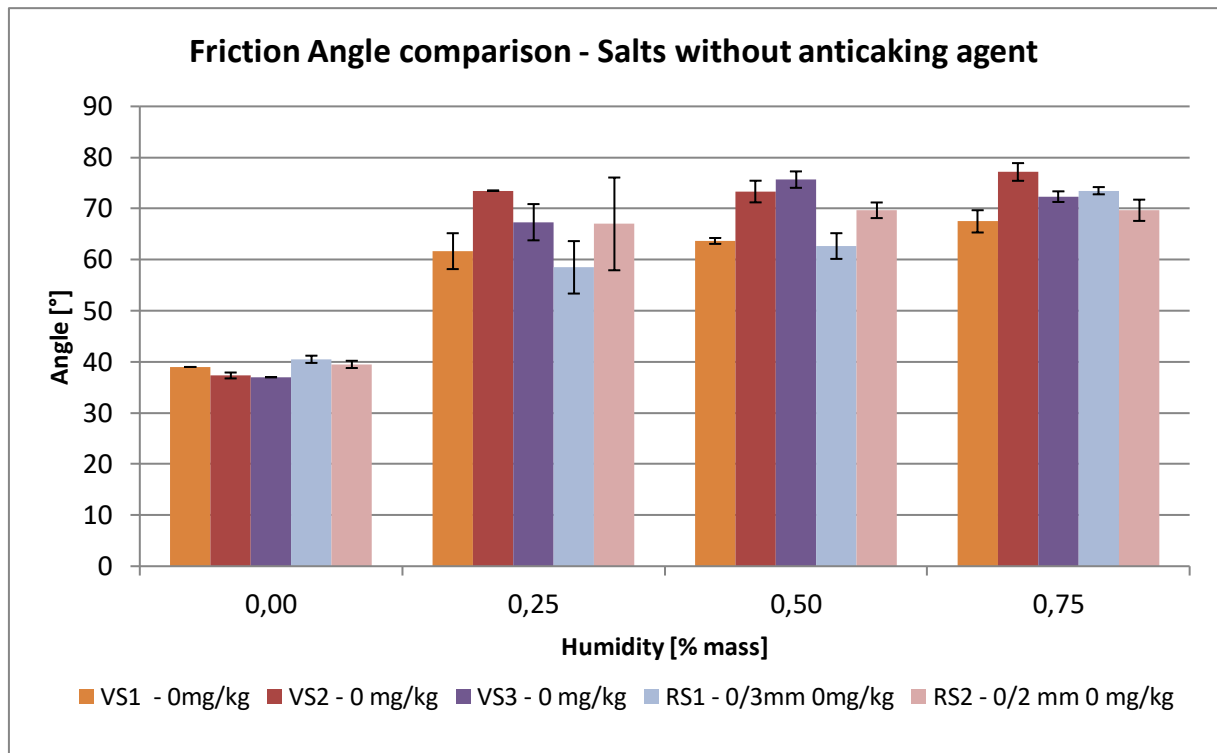
Figure 54: Friction angle results comparison for salts without anticaking agent
