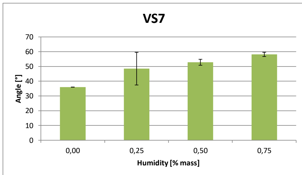
Figure 43: Friction Angle results for VS7
