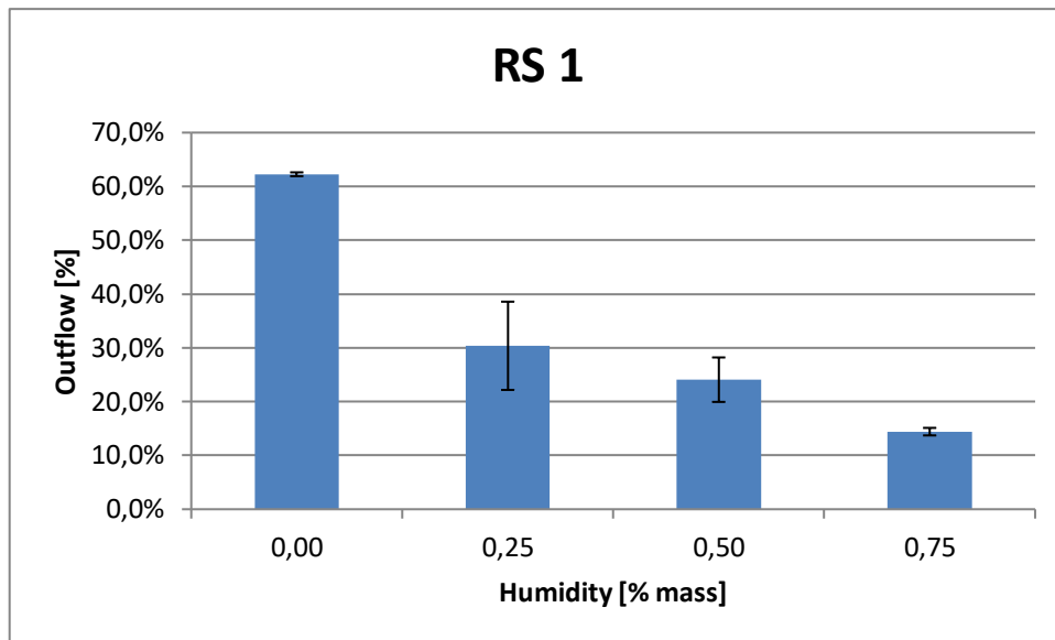
Figure 15: Outflow ratio results for RS1
