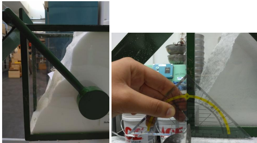
Figure 13. Problems with measurement of internal friction angle
