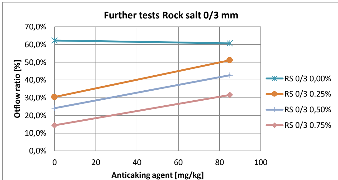
Figure 59: Outflow ratio for RS 0/3 mm depending on the amount of SFC for humidities 0,00 %; 0,25 %; 0,50% and 0,75%
