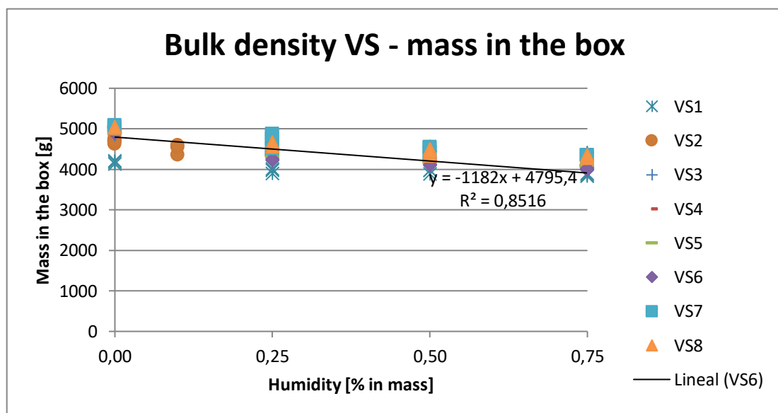
Figure 58: Bulk density results from vacuum salt
