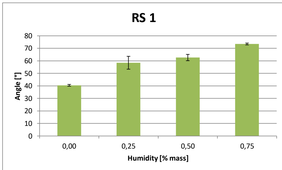
Figure 16: Friction angle results for RS1
