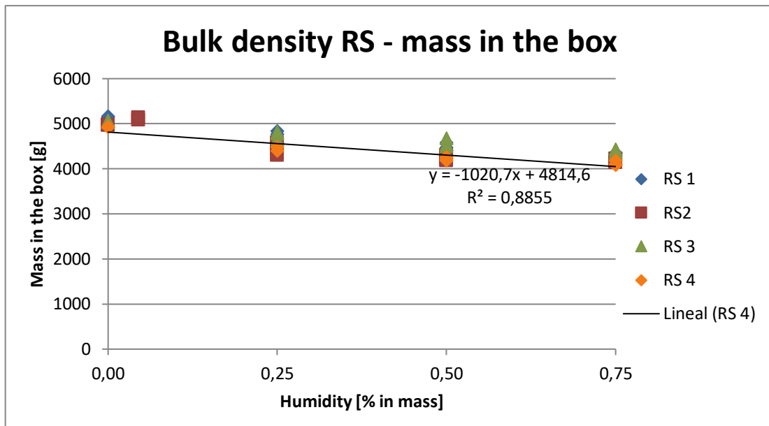
Figure 57: Bulk density results from rock salt
