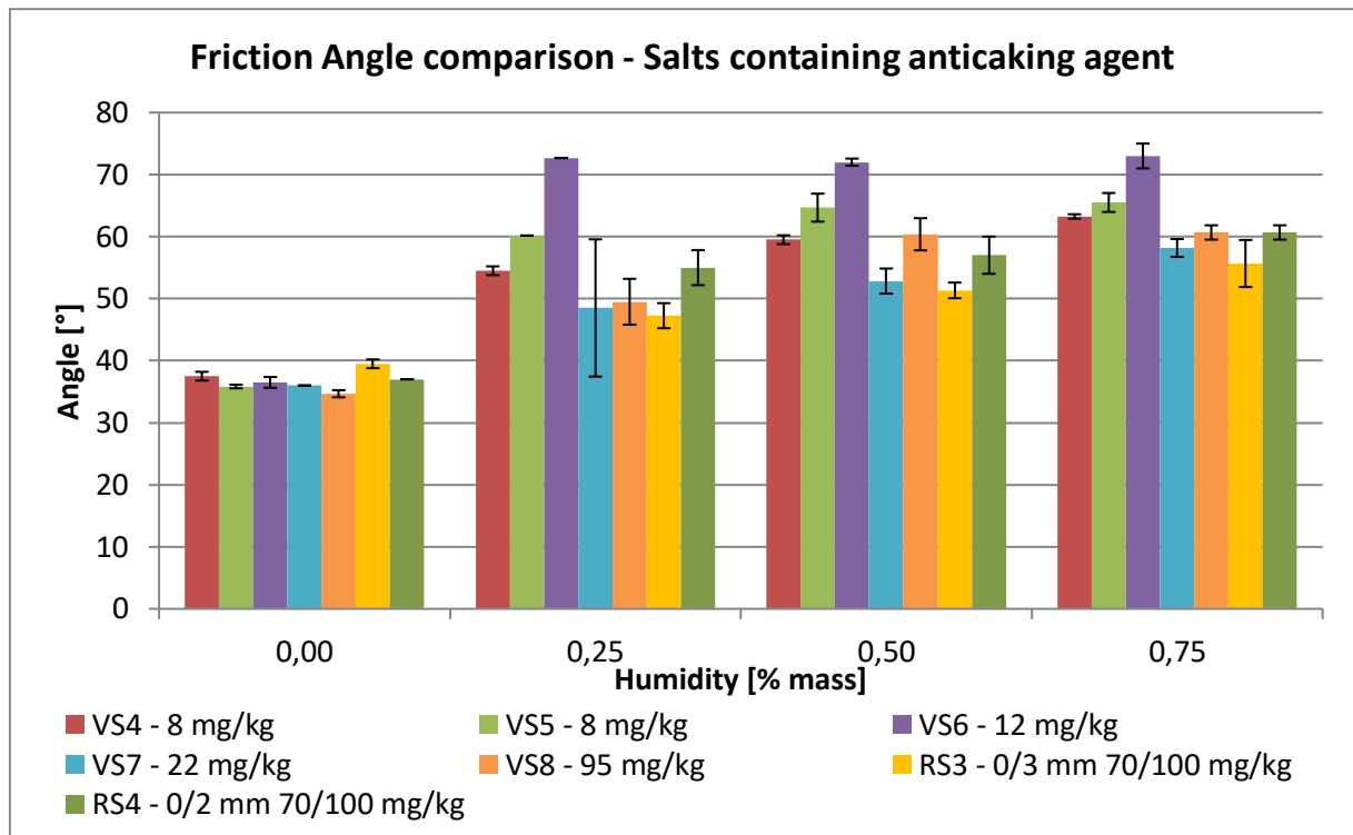
Figure 56: Friction angle result comparison for samples containing anticaking agent
