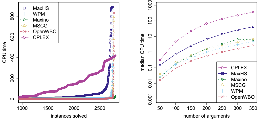
Figure 12: MaxSAT solver comparison for NP-complete strict extension enforcement under the complete semantics.
