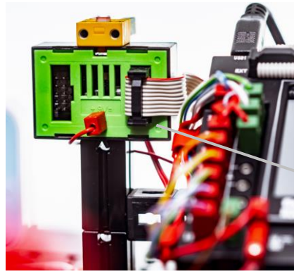
Sensorstation
