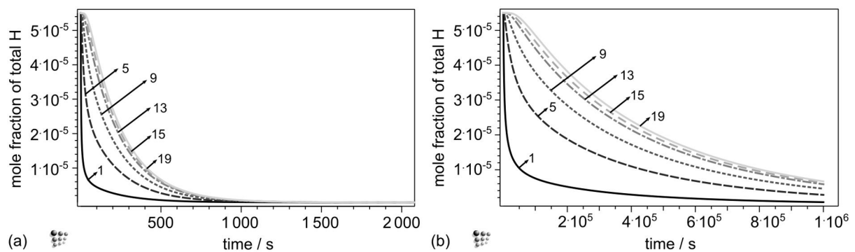
Figure 7: Discharging kinetics for selected cells a) without traps and b) in the presence of NbC-precipitates ( \Delta E = 37 kJ/mol); the y-axis shows the total H-content in the sample.
