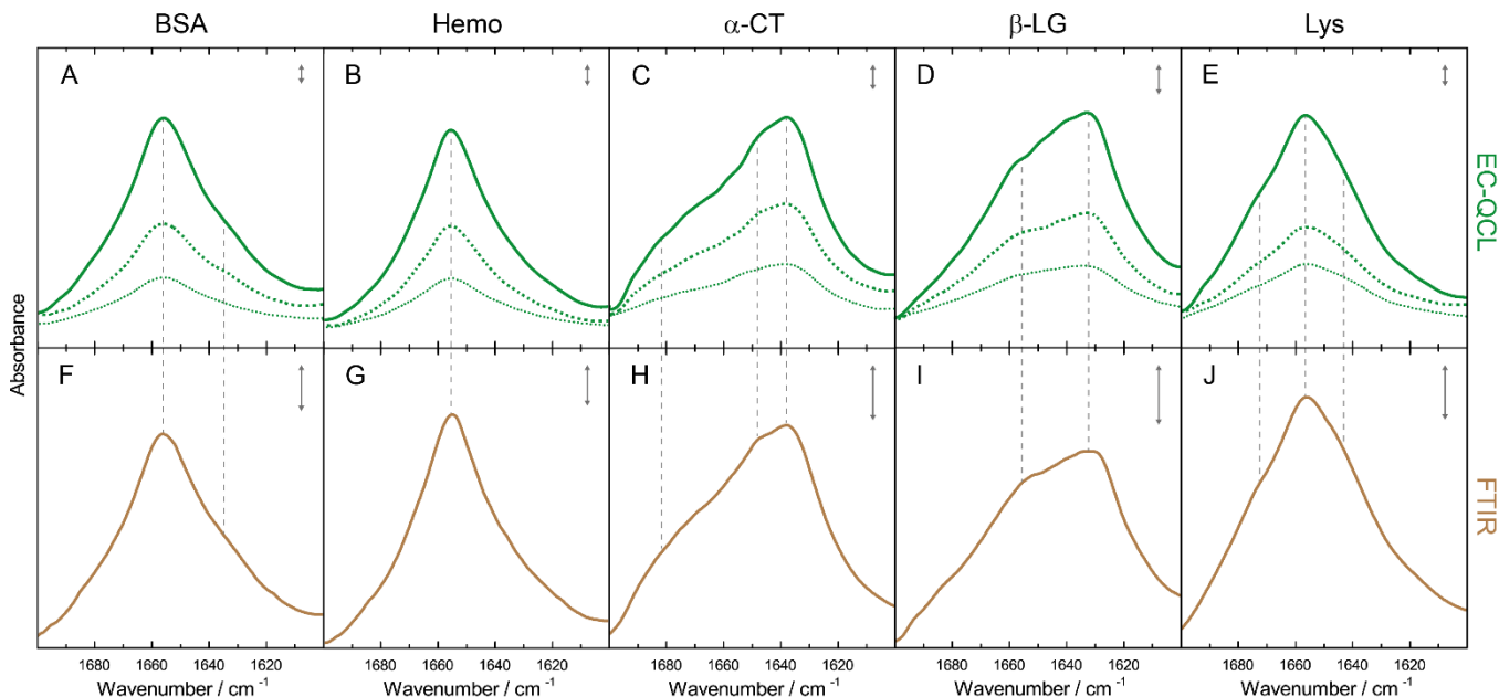
Figure 3. IR absorbance spectra of 10 (green solid line), 5 (green dashed line) and 2.5 mg mL -1 (green dotted line) protein solutions acquired by the EC-QCL setup (A-E) and 20 mg mL -1 (brown solid line) protein solutions acquired by FTIR spectroscopy (F-J). Grey dashed lines highlight the high congruence of the spectral features between the IR spectra acquired by EC-QCL and FTIR spectroscopy. Grey double-headed arrows indicate the absorbance of 10 mAU.
