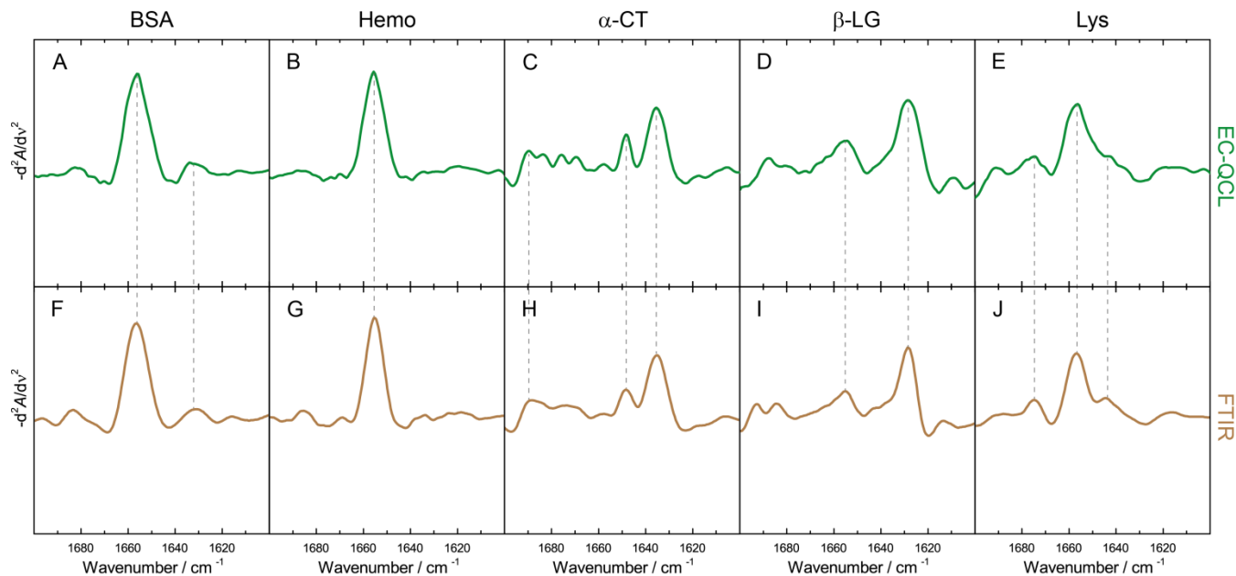
Figure 4. Inverted second derivative spectra of sample proteins acquired by the EC-QCL setup (A-E) and FTIR spectroscopy (F-J). Grey dashed lines highlight the high overlap of the spectral features between the IR spectra acquired by EC-QCL and FTIR spectroscopy.
