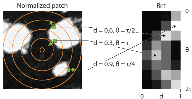
Figure 3.20: Construction of a RIFT descriptor: sample points in the normalized patch (left) transformed into different locations in the descriptor (right). (Figure taken from [80])
