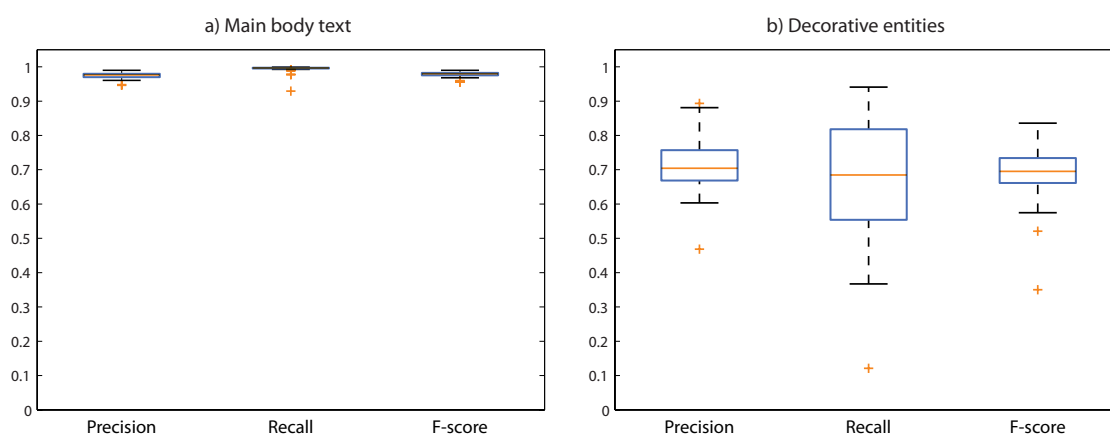
Figure 5.7: Localization evaluation per image.
