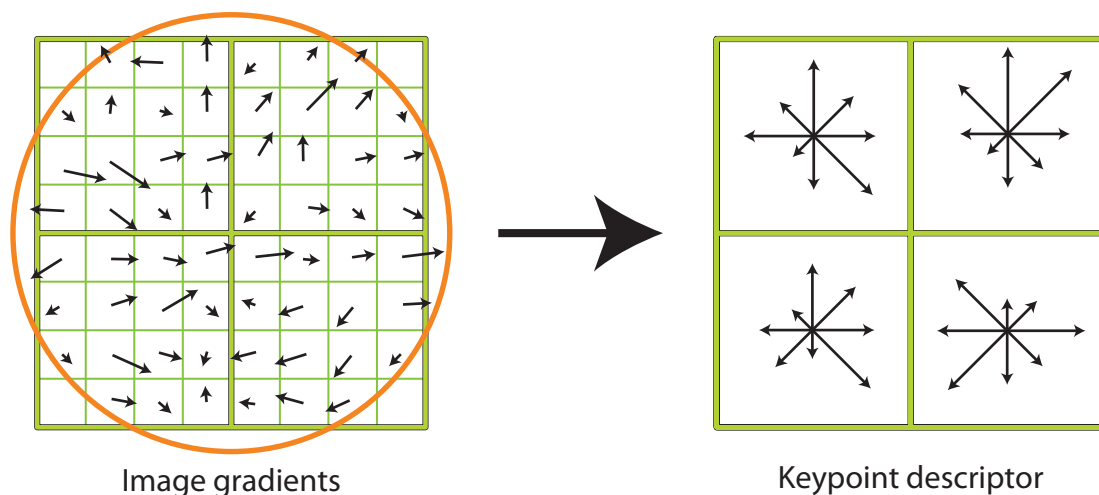
Figure 3.26: Construction of a SIFT descriptor, where for the ease of illustration, a 2 \times 2 descriptor is shown. A sample with gradient orientations and magnitudes is shown (left), where the Gaussian window weighting the magnitudes is indicated by the orange circle. The gradients are then accumulated to an orientation histogram having bins (right). (Figure taken from [93])
