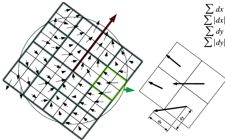
Figure 3.22: Construction of the SURF descriptor: an oriented grid having 4 \times 4 square subregions is established at the interest point (left). The 2 \times 2 grids are the actual fields of the descriptor, where sums dx , |dx| , dy , |dy| are computed with respect to the grid orientation (right). (Figure taken from [14])
