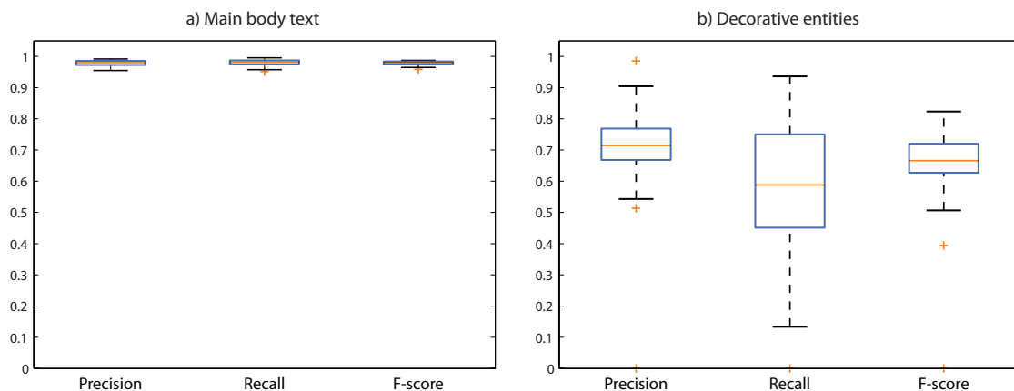
Figure 5.9: Localization evaluation per image.
