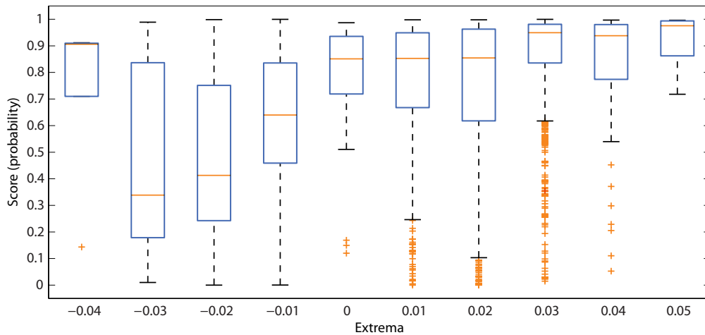
Figure 4.10: Extrema values of the interest points plotted versus their classification score
