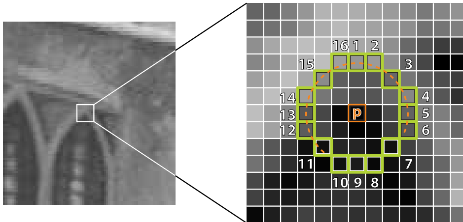
Figure 3.8: FAST uses the highlighted squares (green) at a given radius (orange arc) around the center pixel p (orange) to detect corners. Adjacent pixels brighter than p by a threshold are taken into account for the corner detection (indicated by the orange arc). (Figure taken from [118])
