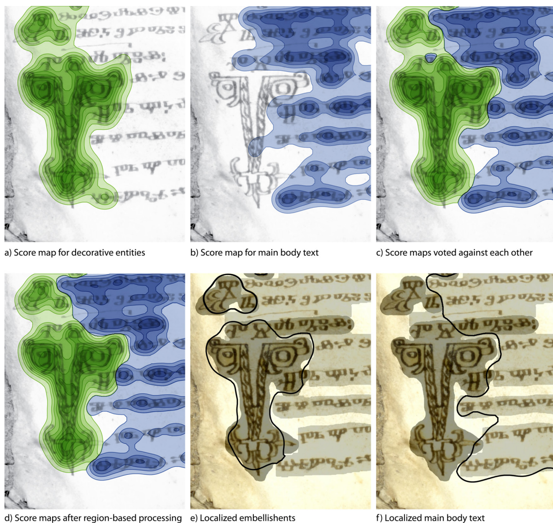
Figure 4.11: Post-processing: both score maps a) and b) are voted against each other resulting in c), a filtering approach rejecting small regions is applied leading to d). e) and f) illustrate the localized entities.
