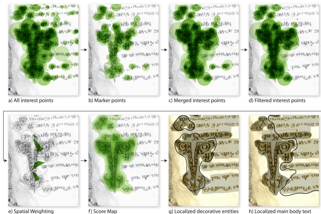
Figure 4.8: Overview of the cascading localization algorithm ( Folio 85r )
