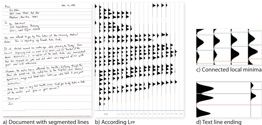
Figure 2.9: LPP (Figure taken from [6])
