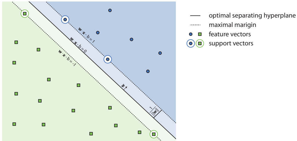
Figure 3.28: Linear separable classes divided by a hyperplane (solid black line) and the maximal margin (dotted line).
