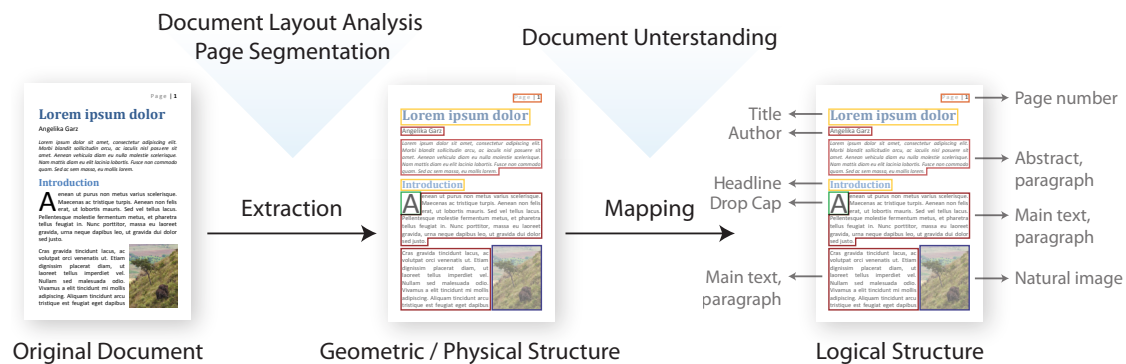
Figure 2.1: Basic model for document image analysis (Figure inspired by [131])
