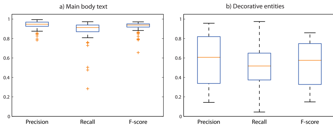
Figure 5.3: Localization evaluation per image.
