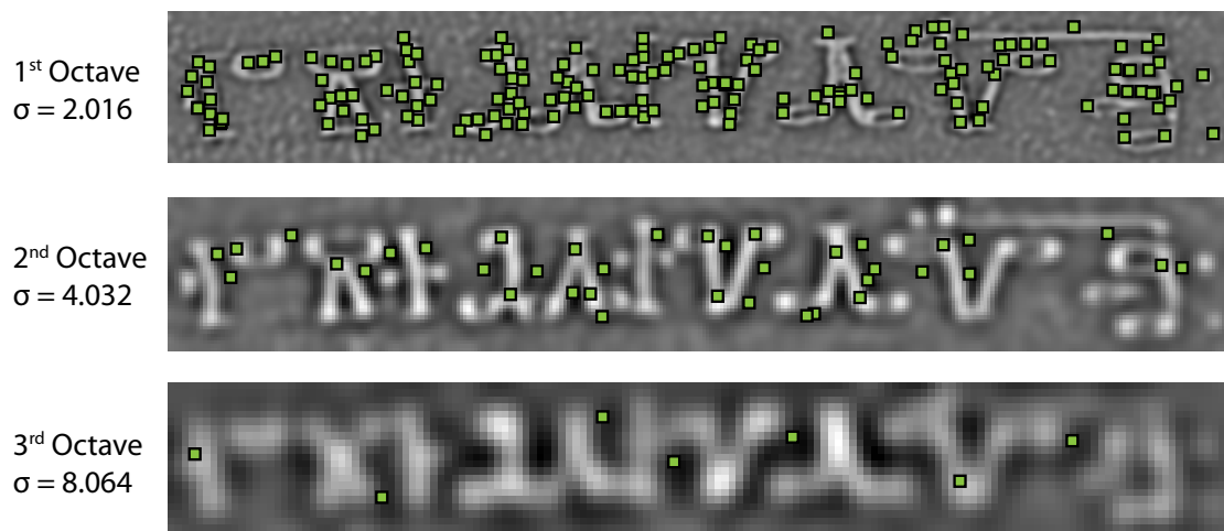
Figure 4.3: The first representations of each octave with \sigma given are overlaid with interest points detected in the DOG scale space which denoted by green squares.
