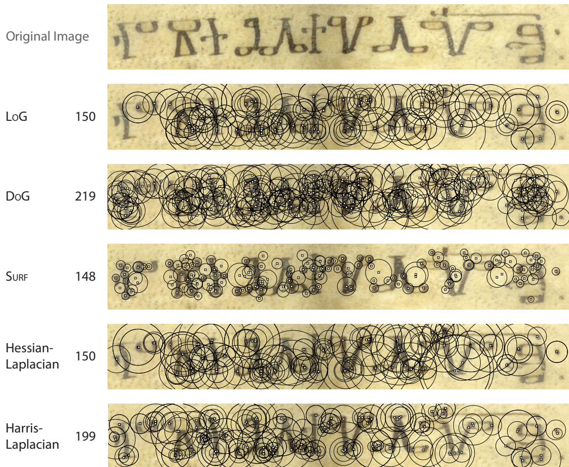
Figure 4.2: Comparison of five potential scale-invariant interest point detectors (four blob detectors: LOG, DOG, SURF, Hessian-Laplacian, one corner detector: Harris-Laplacian) on a heading of the Psalter dataset. The numbers in column Points denotes the number of Interest Points extracted with the respective interest point detector.
