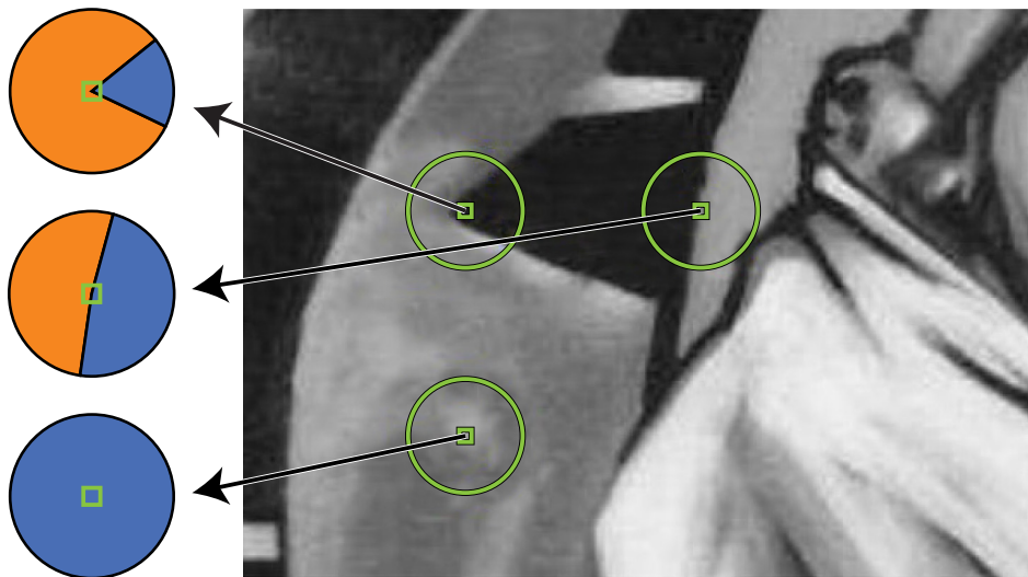
Figure 3.3: Interest points detected by the SUSAN corner detector. The neighborhood is divided into “similar” (orange) and “dissimilar” (blue). Corners are characterized by a minimum area of “similarity” (Figure taken from [134])
