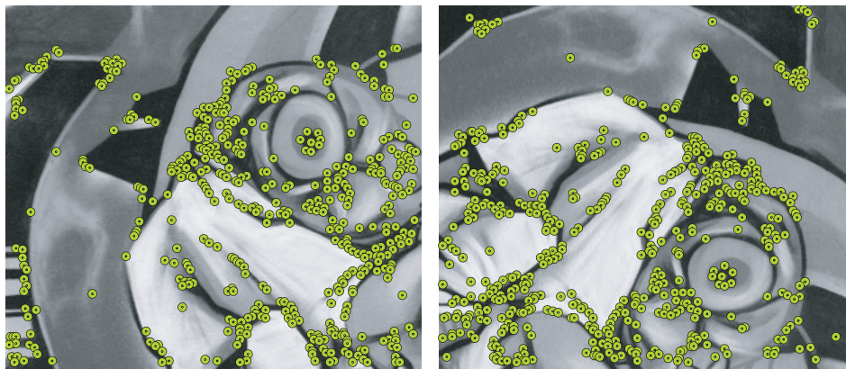
Figure 3.9: Corresponding interest points found in both image using the FAST detector (Figure taken from [134])
