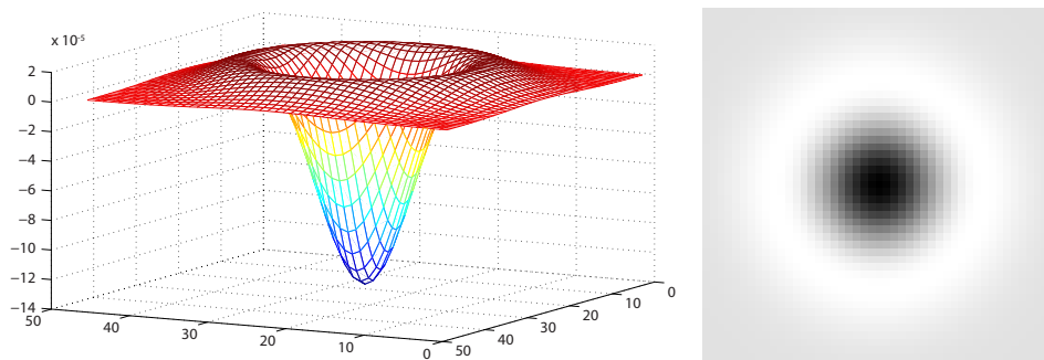
Figure 3.10: LOG as 3D Plot (left) with color coding, and in normalized gray scale coding (right)
