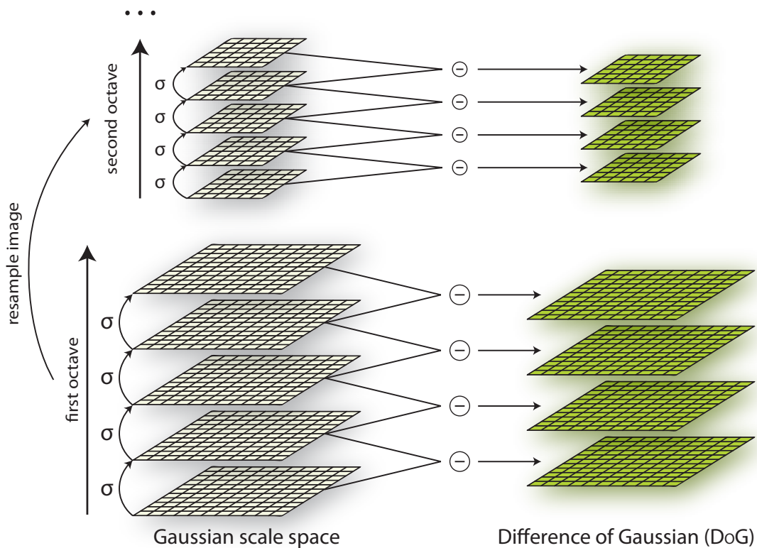
Figure 3.17: Computation of the DOG (Figure taken from [93, 134])
