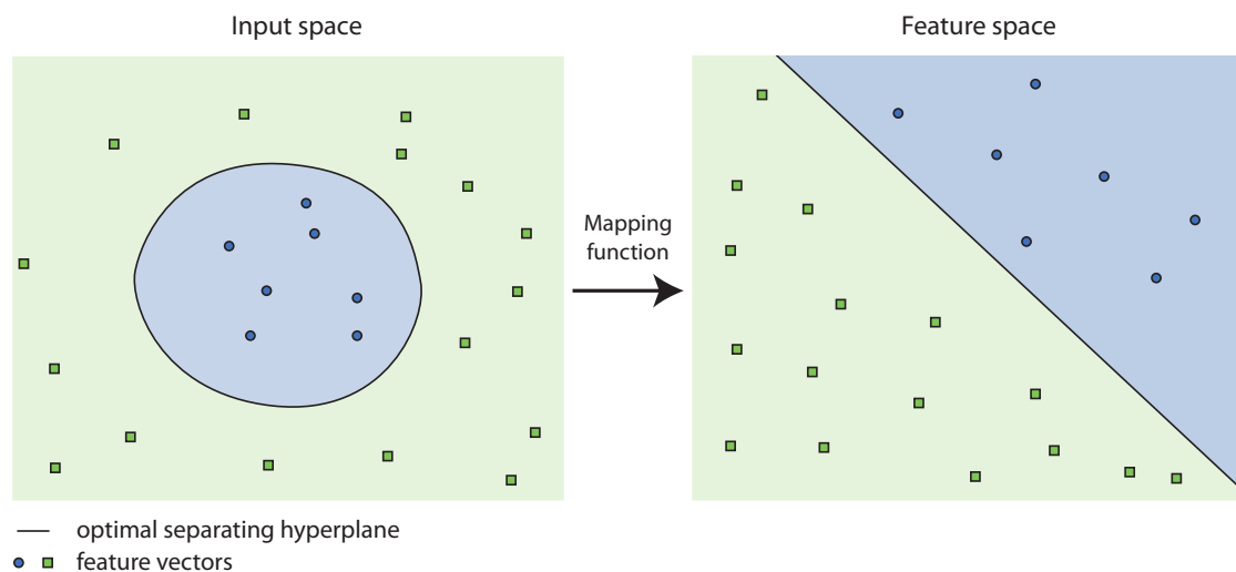
Figure 3.29: Kernel trick: mapping the input space onto a feature space through a function.
