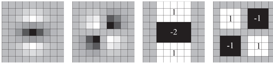
Figure 3.14: Left: The Gaussian second-order partial derivatives ( y -direction and xy ) and their respective SURF equivalents (right). Gray regions are equal to zero. (Figure taken from [15])
