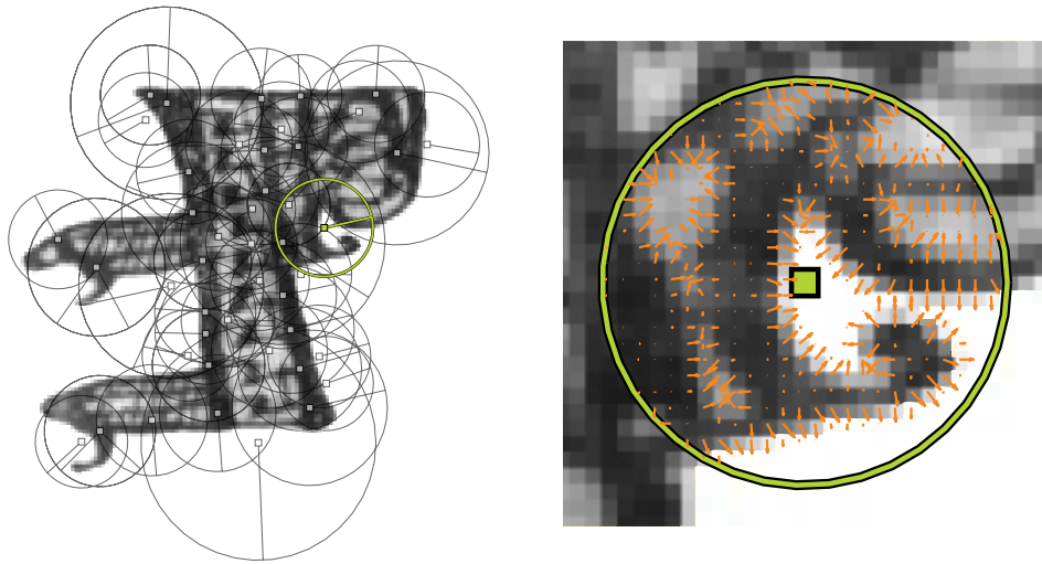
Figure 3.24: Glagolitic decorative initial with overlaid interest points (left). The right side shows a selected interest point (green) with gradients indicated by orange arrows.
