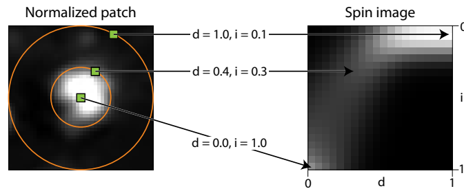
Figure 3.19: Construction of a spin image: sample points in the normalized patch (left) transformed into different locations in the spin image (right). (Figure taken from [81])
