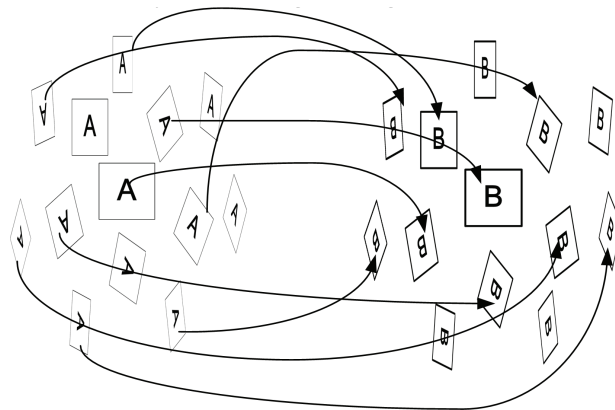
Figure 3.21: ASIFT Algorithm: pairs of rotated and tilted representations obtained from images A and B are compared by SIFT. (Figure taken from [143])
