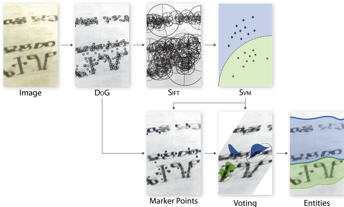
Figure 4.1: Workflow of the proposed layout analysis method showing the main tasks: feature extraction and classification (top) and localization (bottom)
